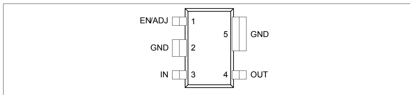
Figure 2 Pin configuration
