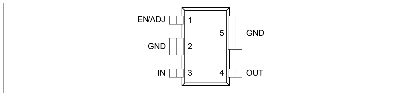
Figure 2 Pin configuration
