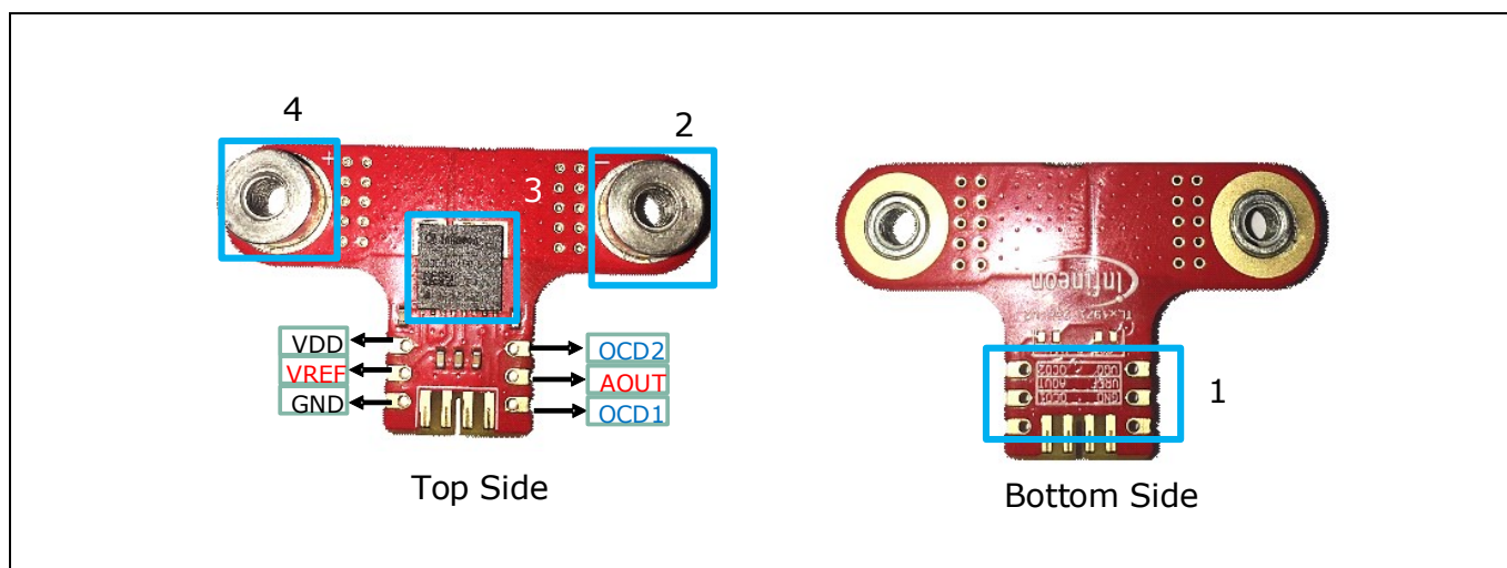
Figure 10 Sensor Board Top and Bottom View
