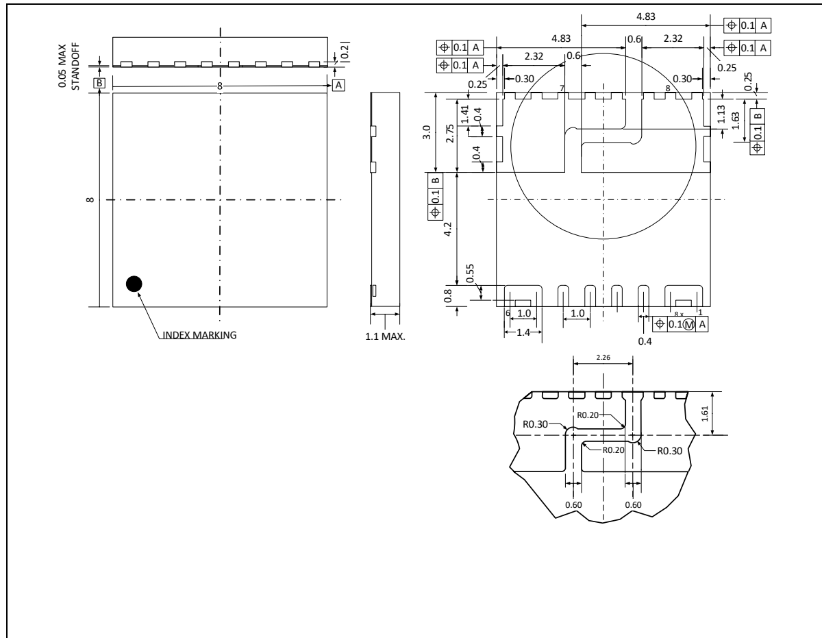
Figure 10 PG-TISON-8 package dimensions
