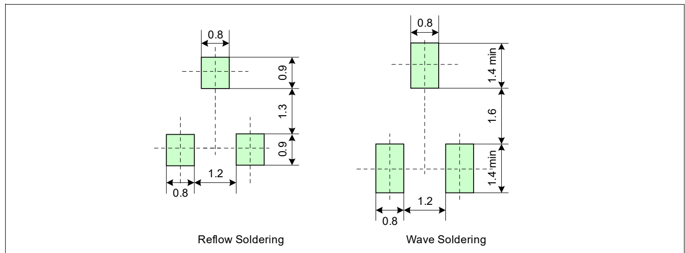
Figure 11 Footprint PG-SOT23-3-15
