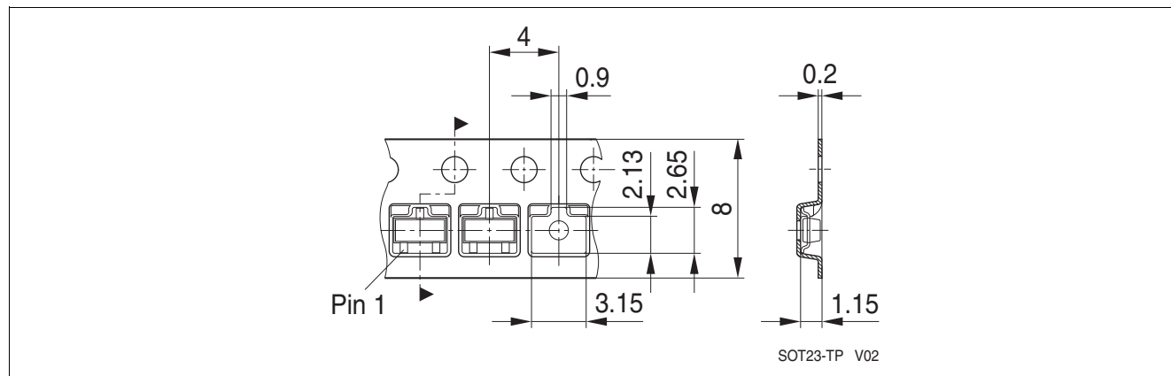
Figure 10 Packing of the PG-SOT23-3-15 in a tape
