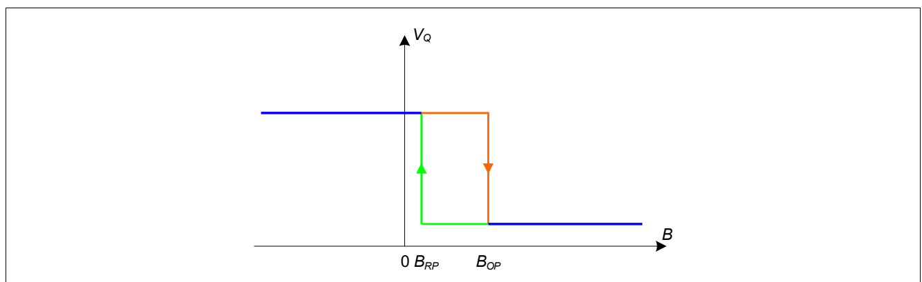
Figure 5 Output signal TLI4965-5M
