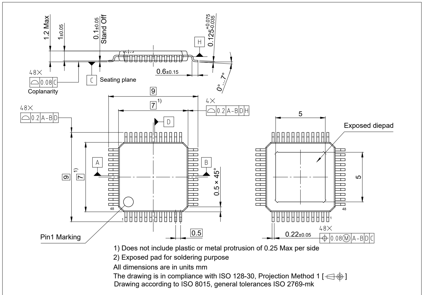
Figure 2 PG-TQFP-48-10
