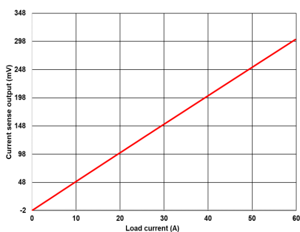
Figure 9 Current sense output
