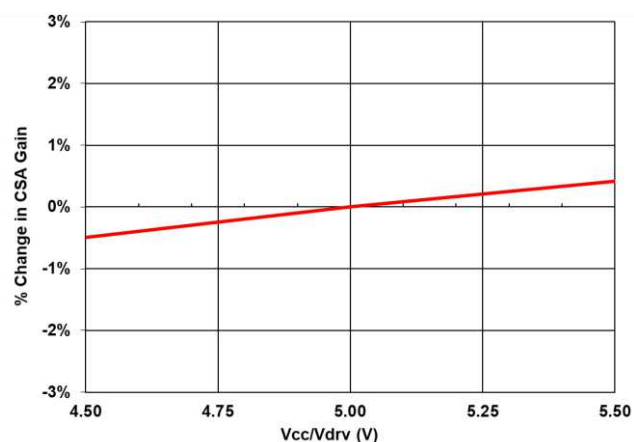
Figure 11 Current sense gain variation vs VCC/VDRV
