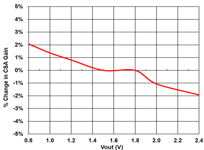
Figure 12 Current sense gain variation vs Vout
