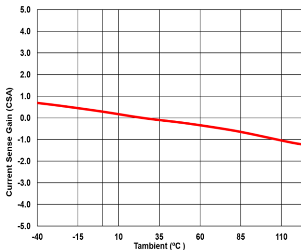
Figure 13 Current sense gain variation vs Temperature
