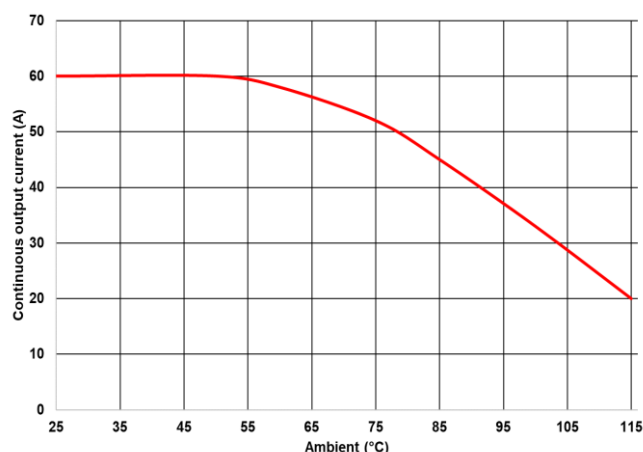
Figure 7 Thermal derating
