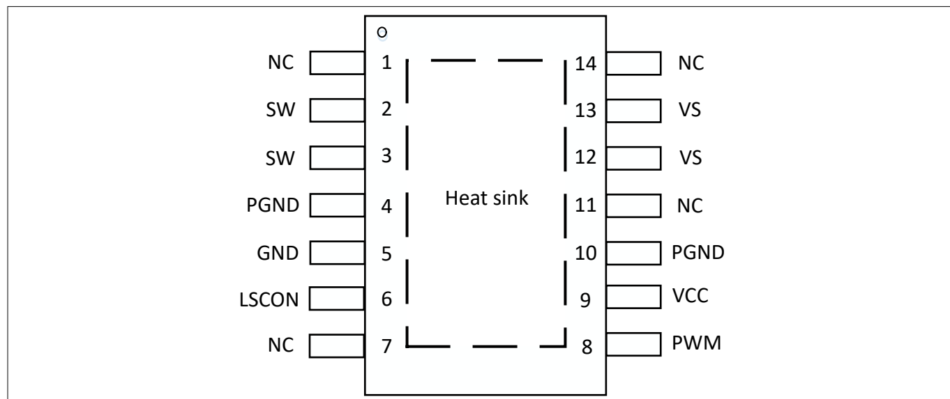
Figure 2 Pin configuration
