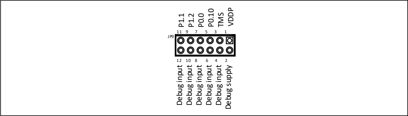
Figure 22 Pinout of JP9
