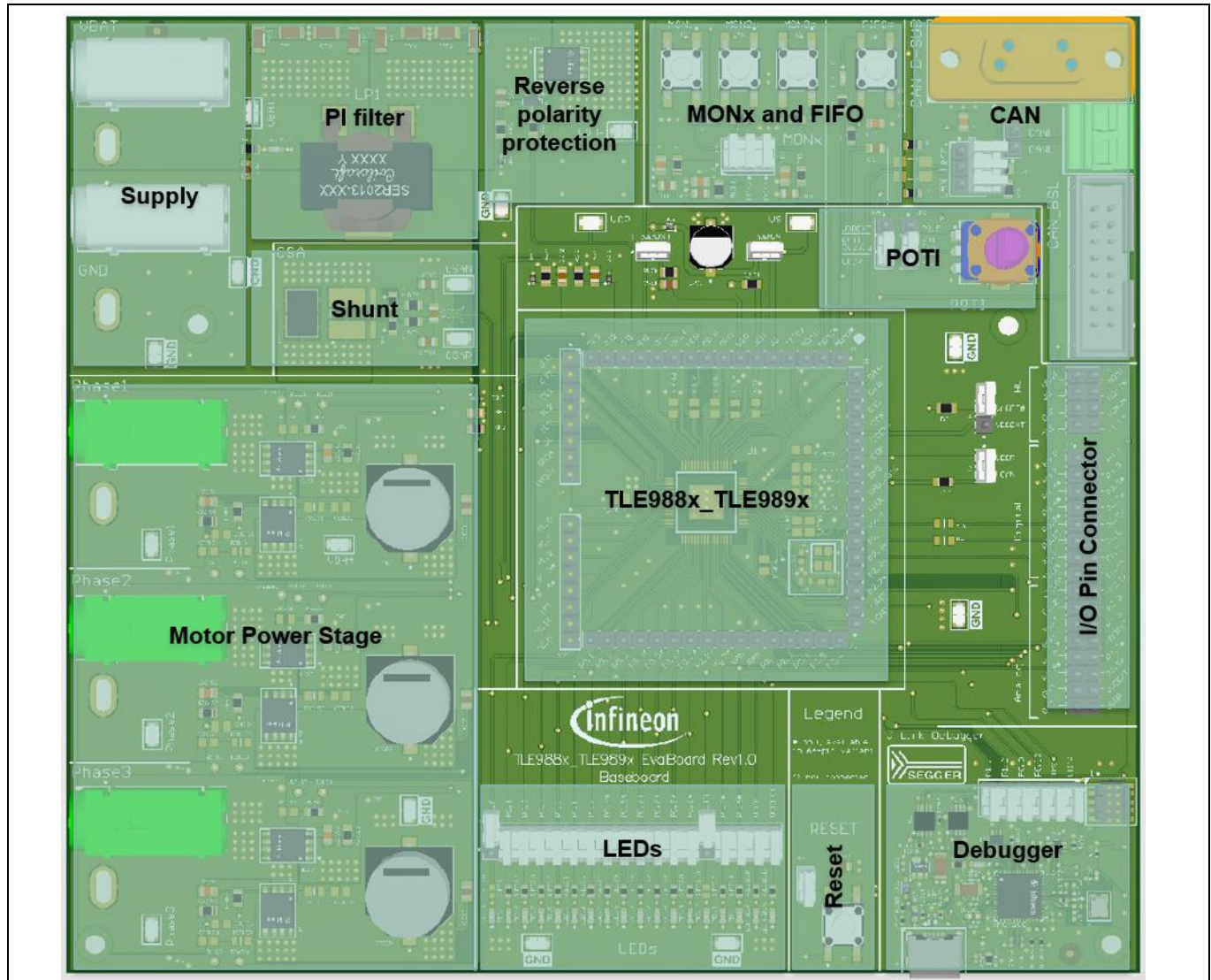
Figure 2 Hardware Implementation
