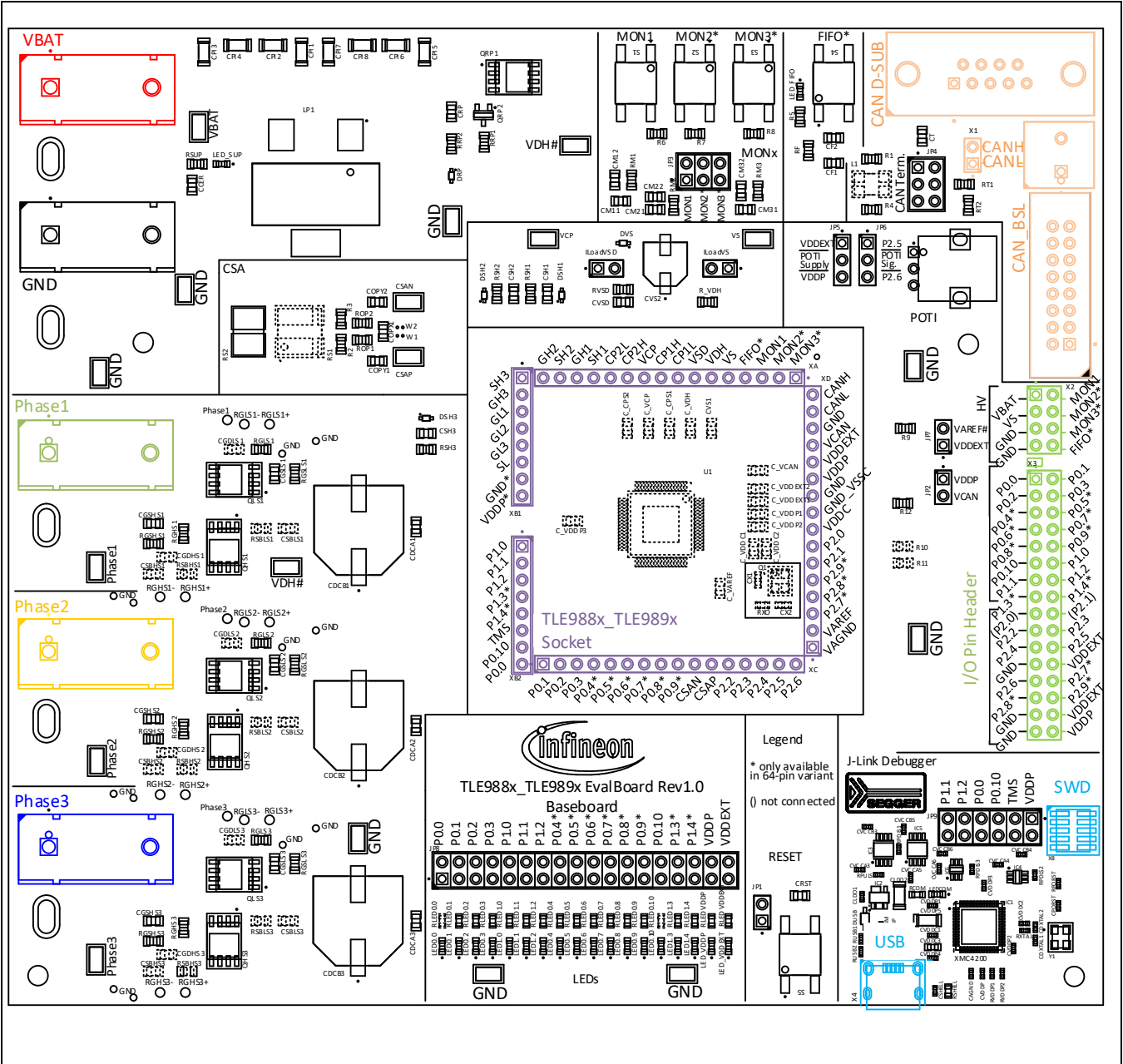
Figure 3 Connectors
