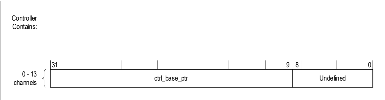
Figure 50 CTRL_BASE_PTR Register Bit Assignments
