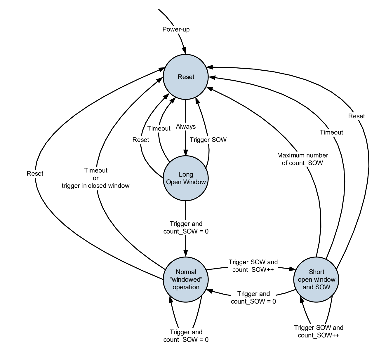
Figure 68 Watchdog timer behavior
