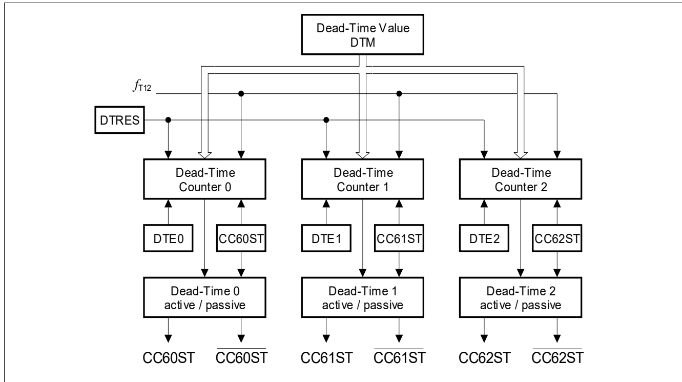
Figure 138 Dead-Time Generation Block Diagram
