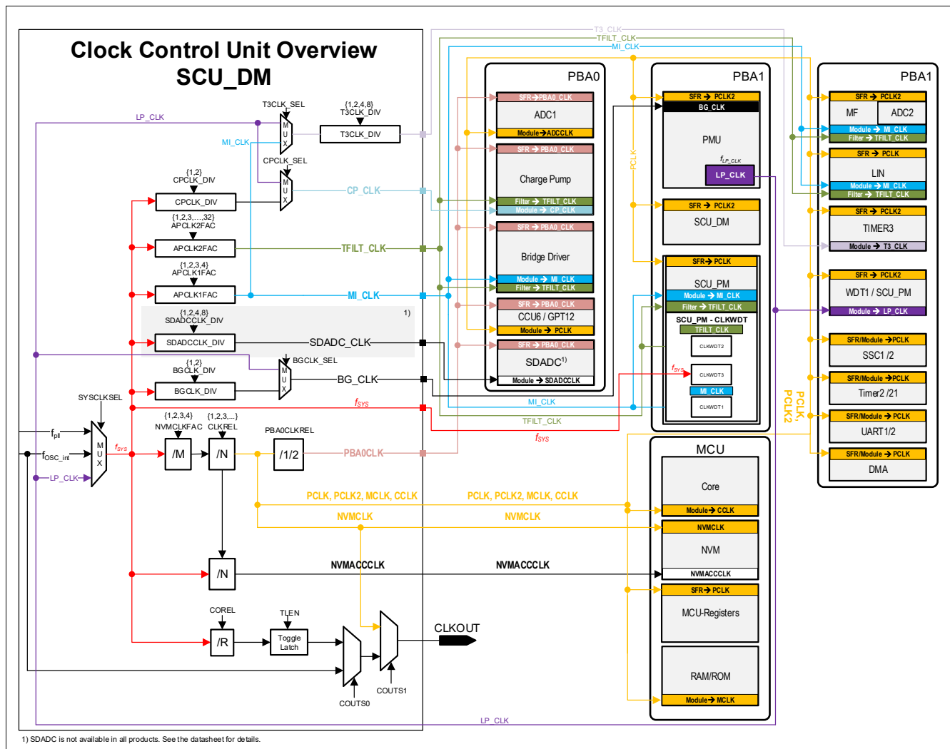
Figure 27 Clock Tree
