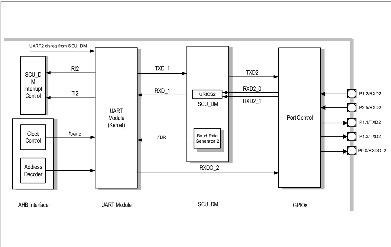
Figure 177 UART2 Module I/O Interface
