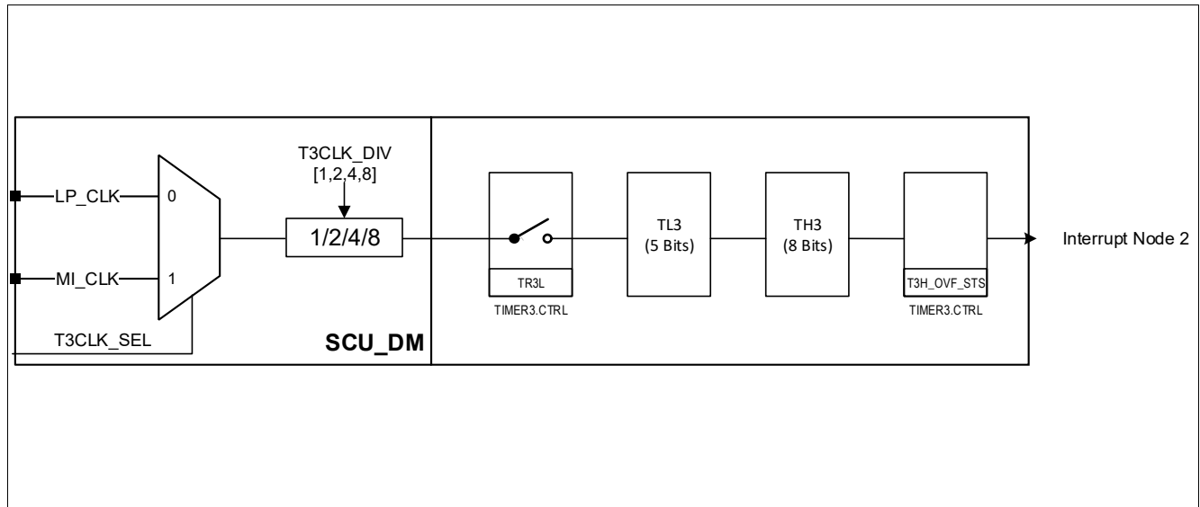
Figure 117 Timer3, Mode 0: 13-Bit Timer
