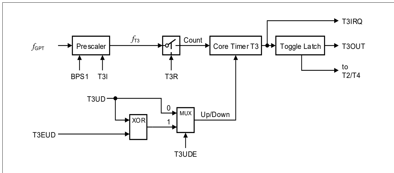
Figure 84 Block Diagram of Core Timer T3 in Timer Mode
