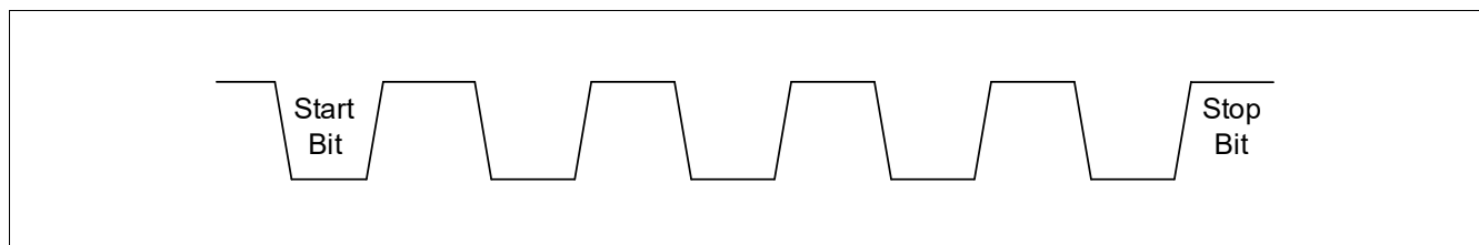
Figure 173 The Synch Byte Field
