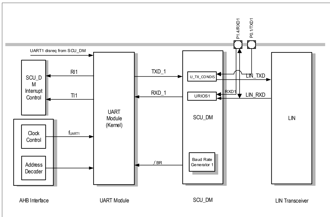
Figure 175 UART1 Module I/O Interface
