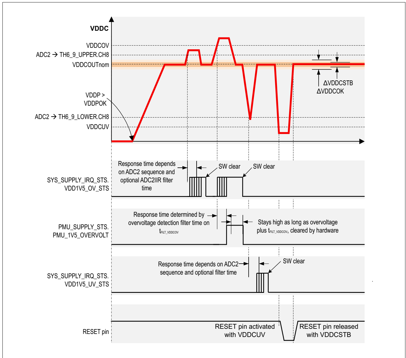
Figure 13 VDDC
