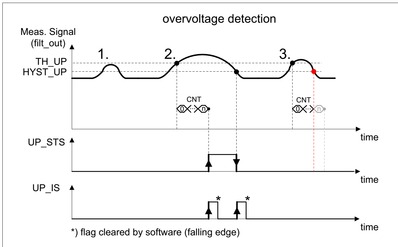
Figure 206 Overvoltage detection
