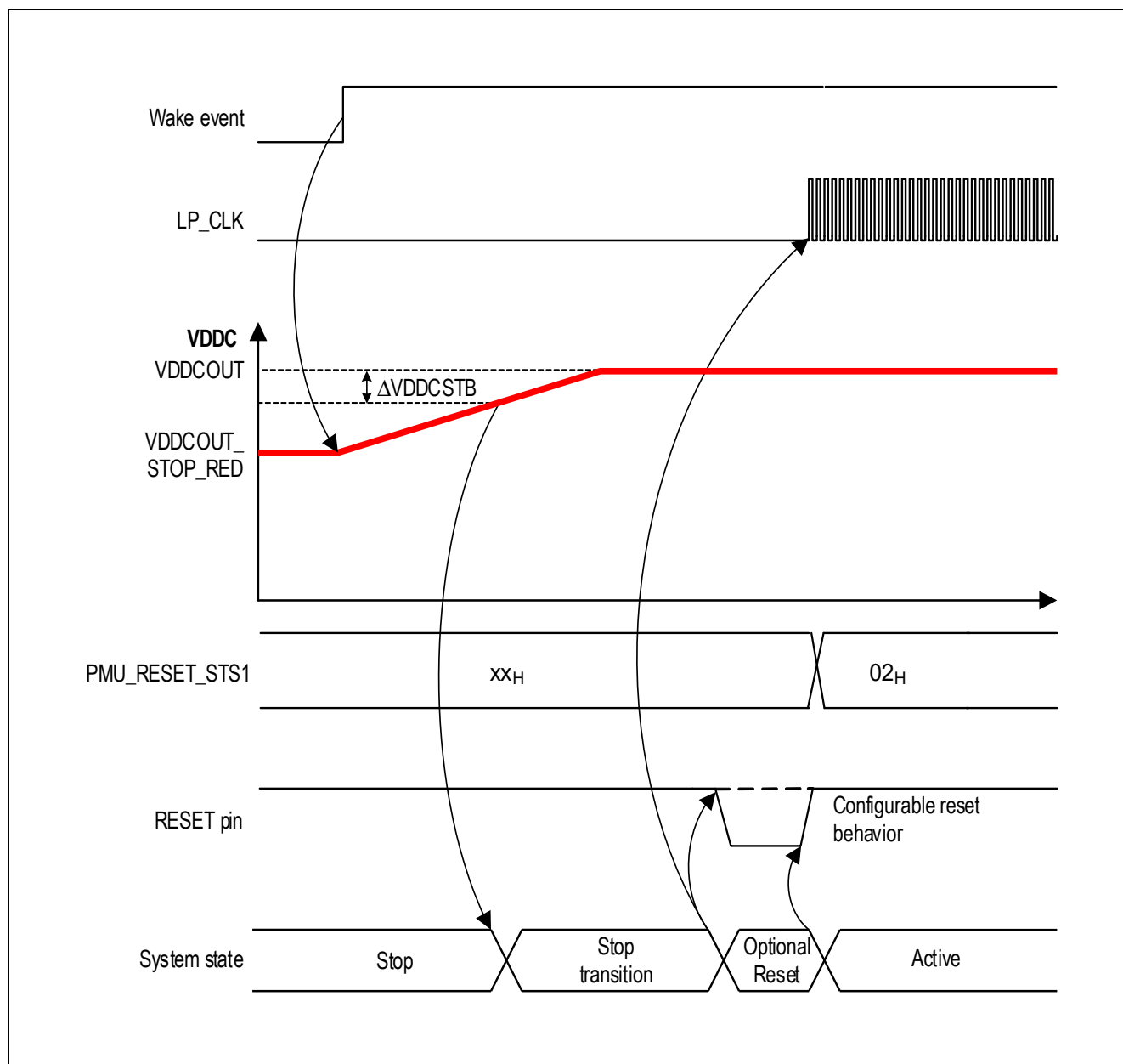
Figure 14 Stop mode exit timing
