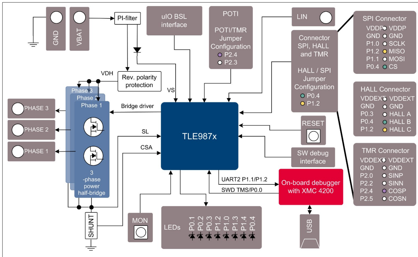
Figure 1 Board concept
