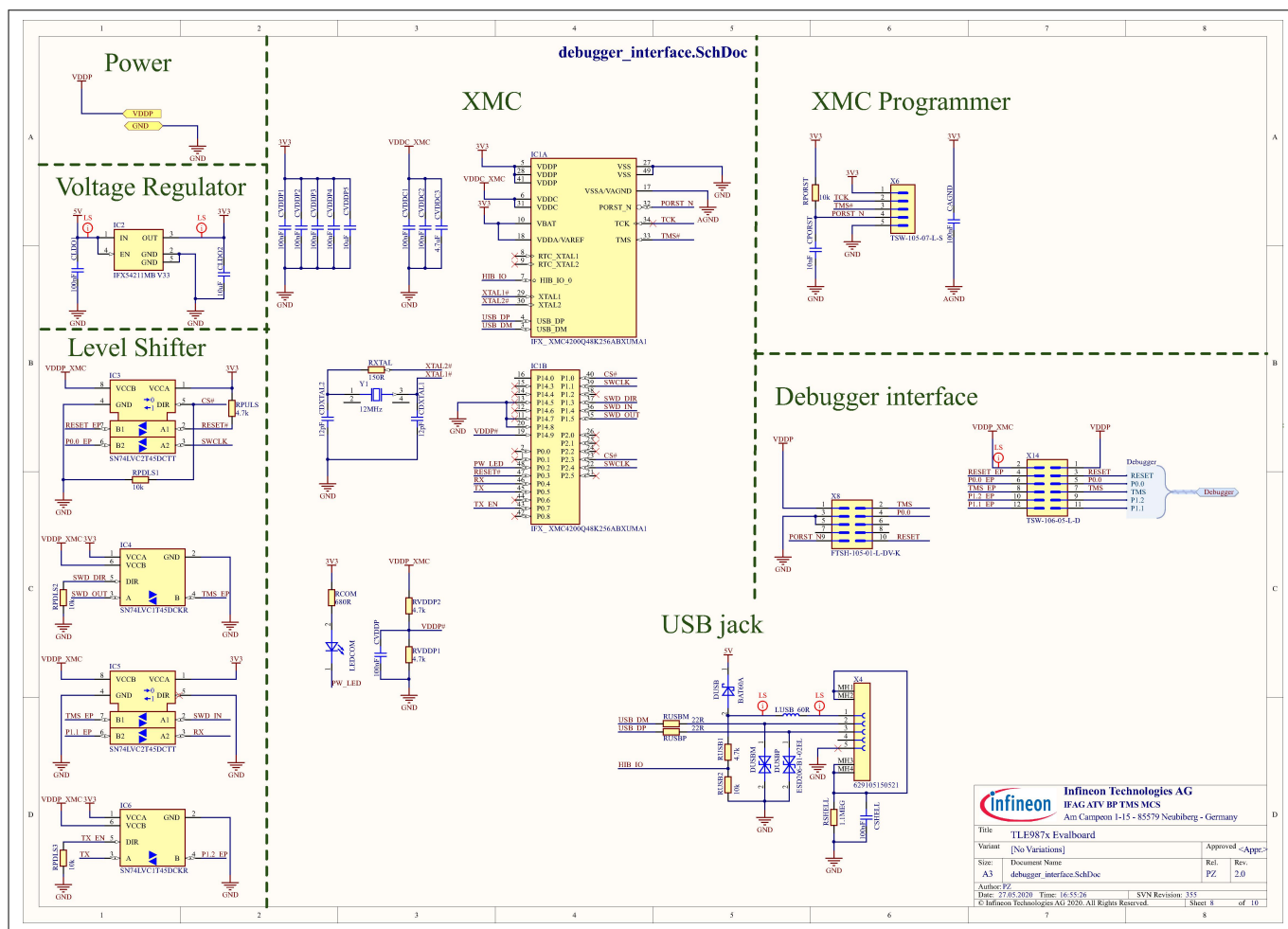
Figure 23 Schematics Sheet 10
