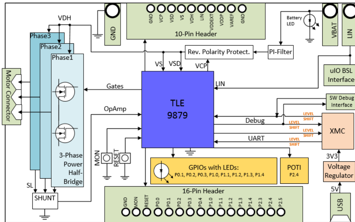
Figure 1: Board Concept
