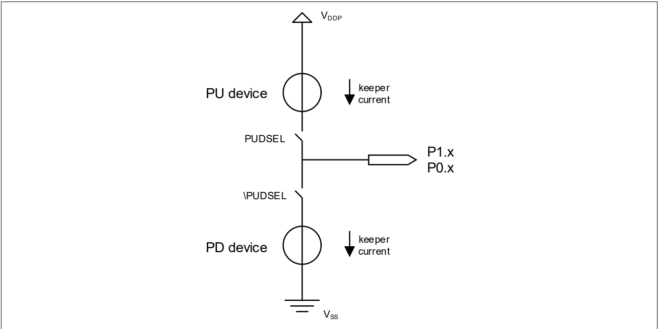
Figure 33 Pull-up/down device
