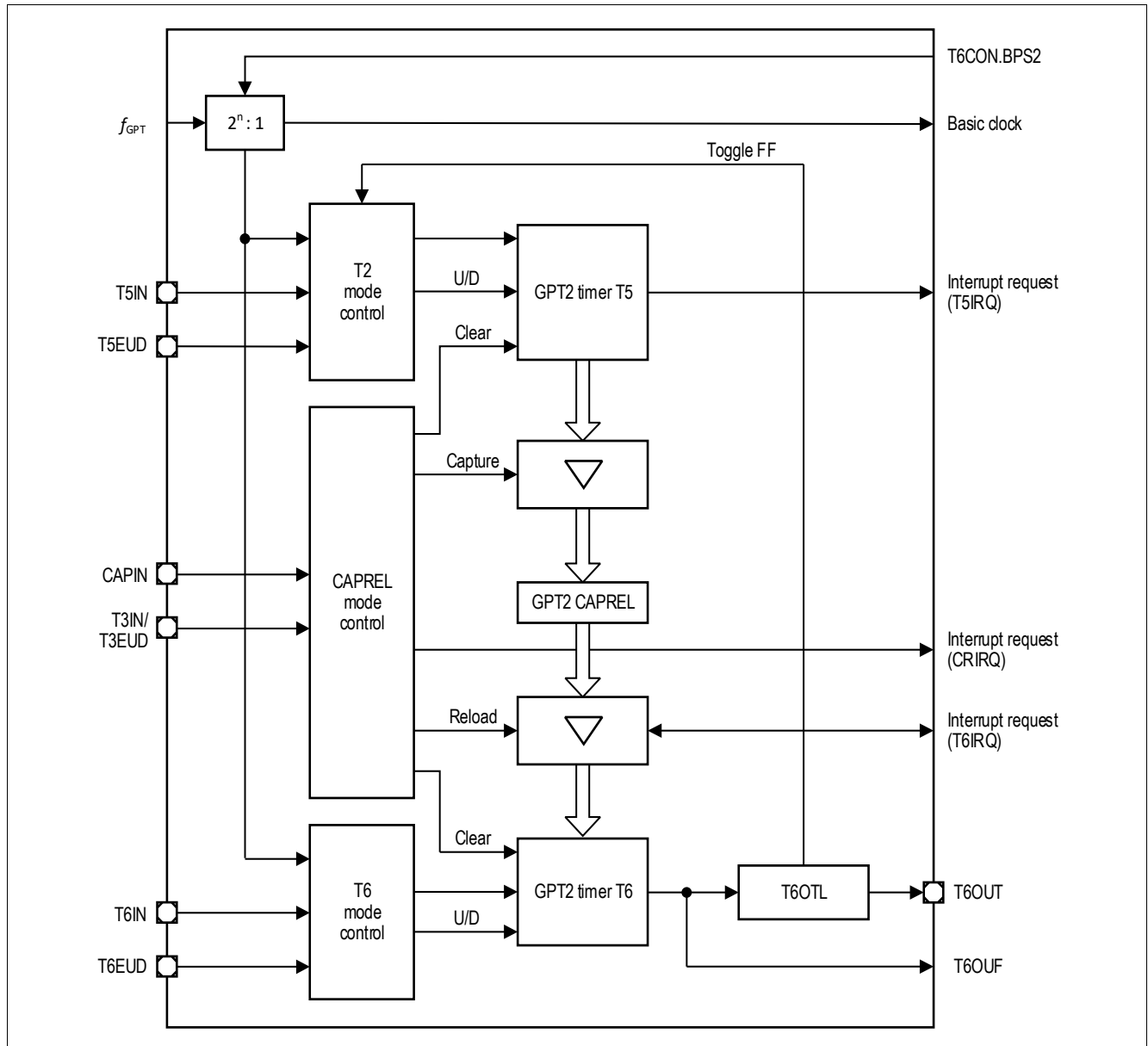
Figure 18 GPT2 block diagram ( n = 1 \dots 4 )
