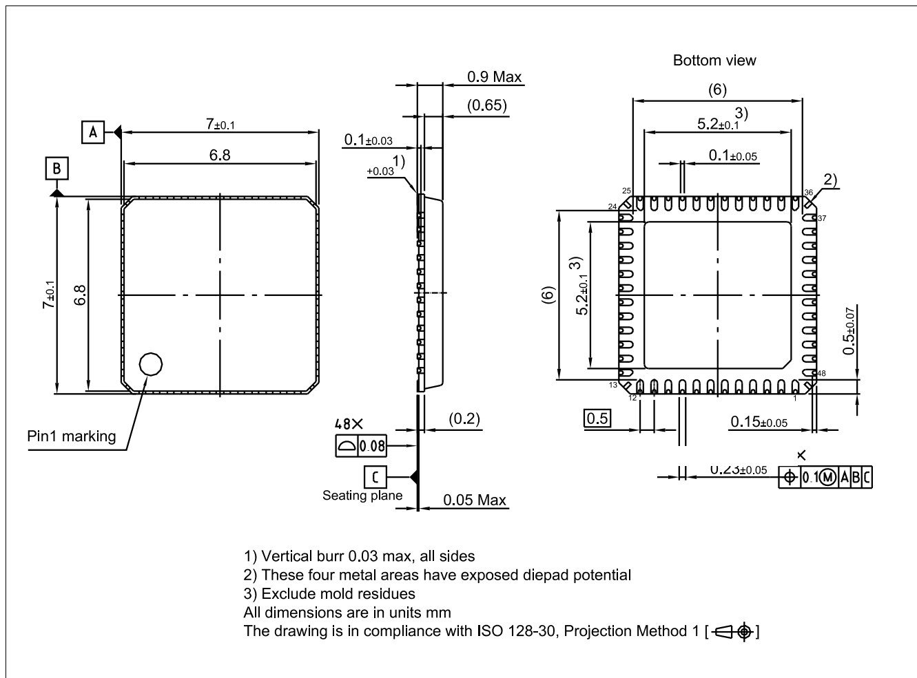
Figure 36 Package outline VQFN-48-29 with LTI (BF step) 1)
