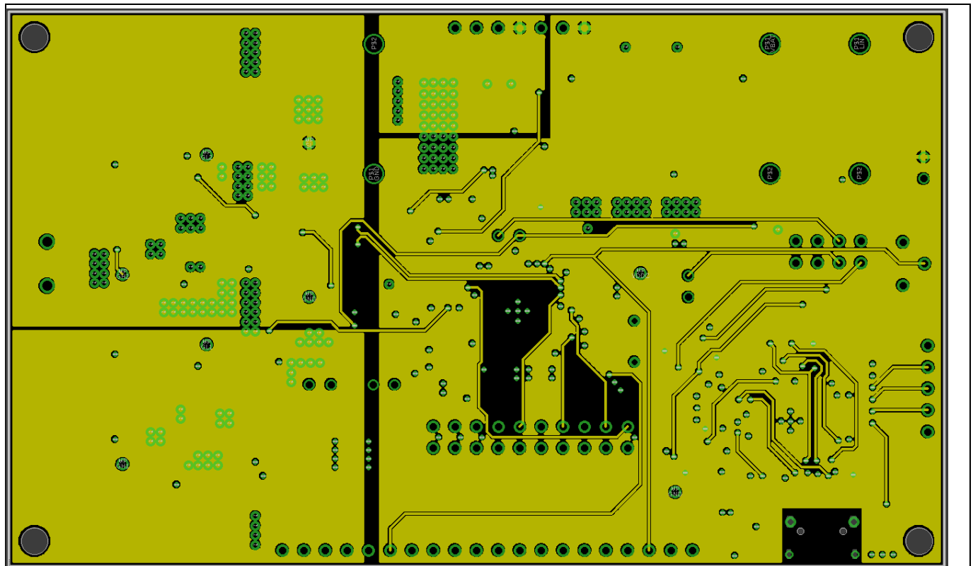
Figure 13 Layout Layer 2
