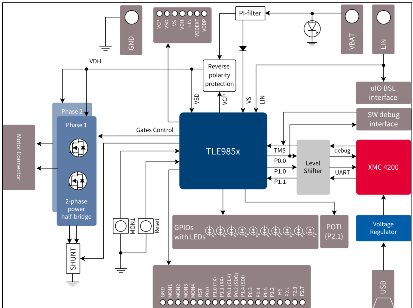
Figure 2 Board Concept
