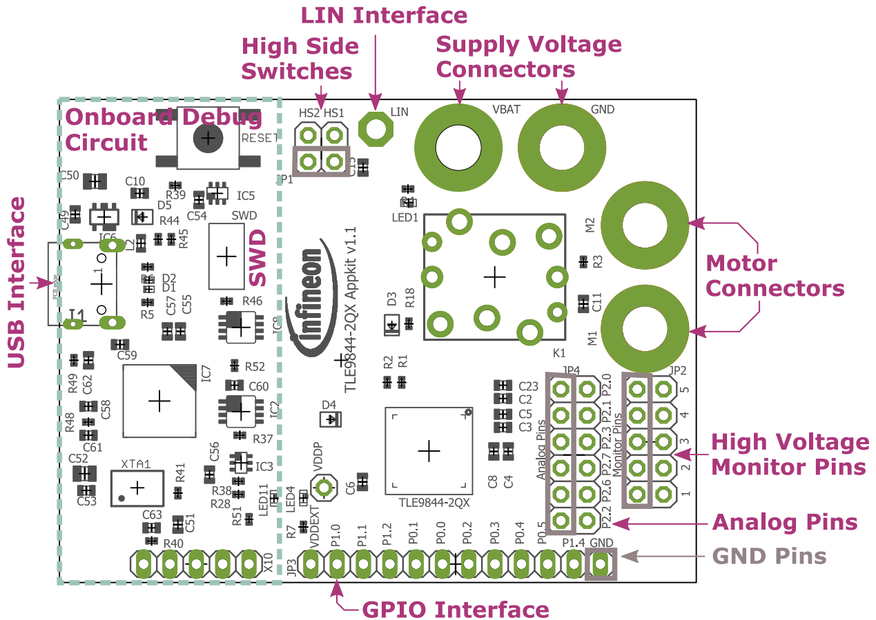
Figure 3 Interconnections Overview
