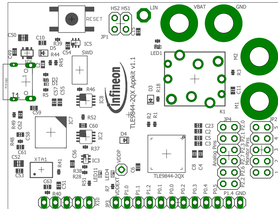
Figure 7 Parts placement
