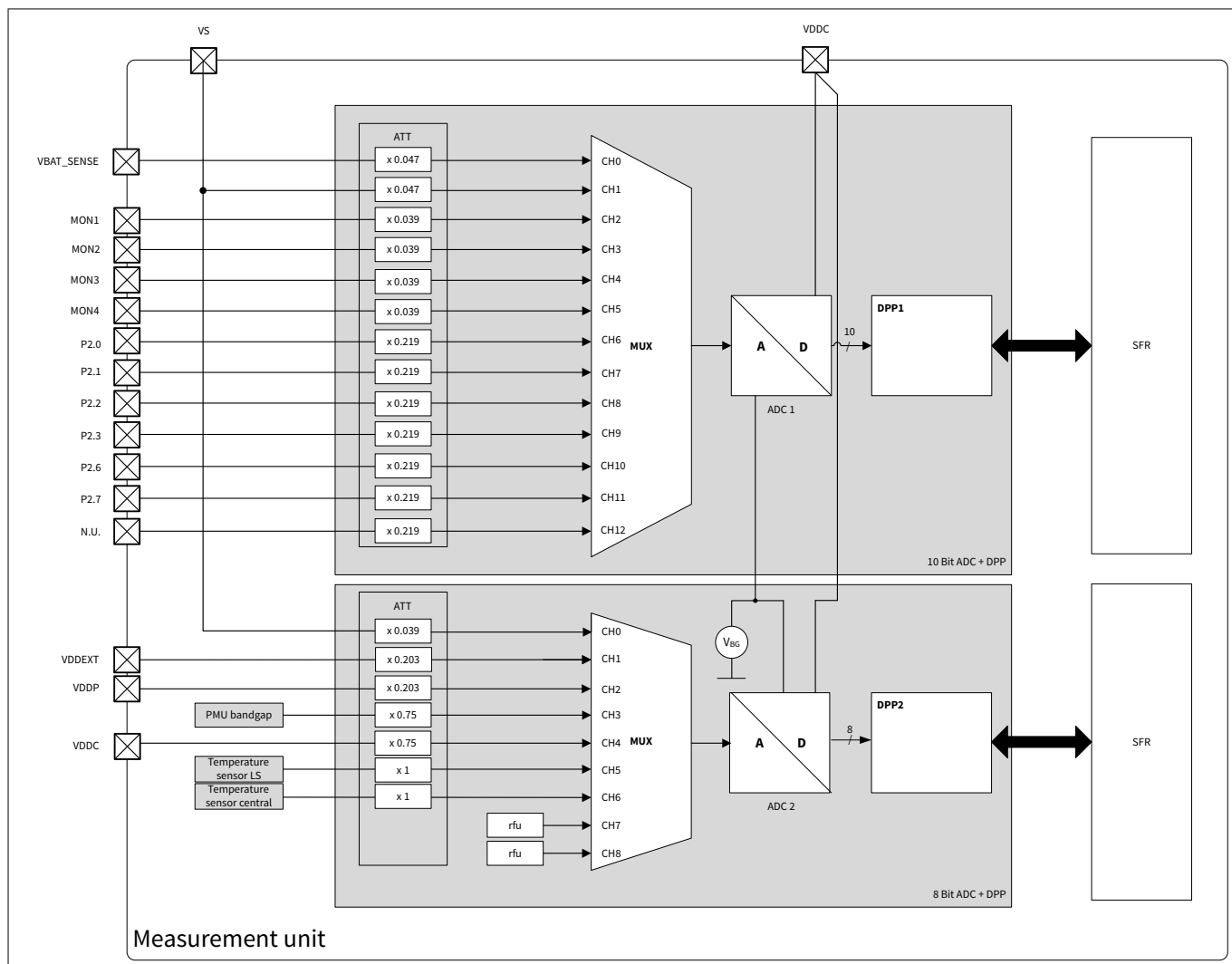
Figure 28 TLE9843QX measurement unit overview
