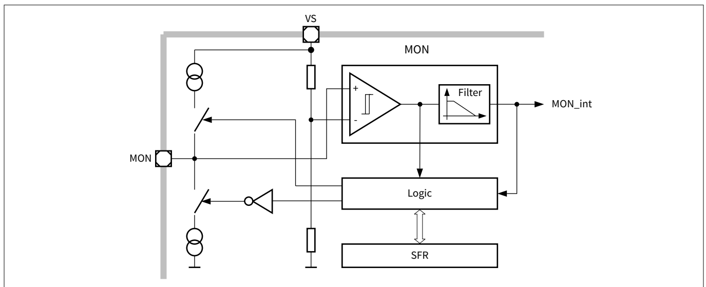
Figure 31 Monitoring input block diagram
