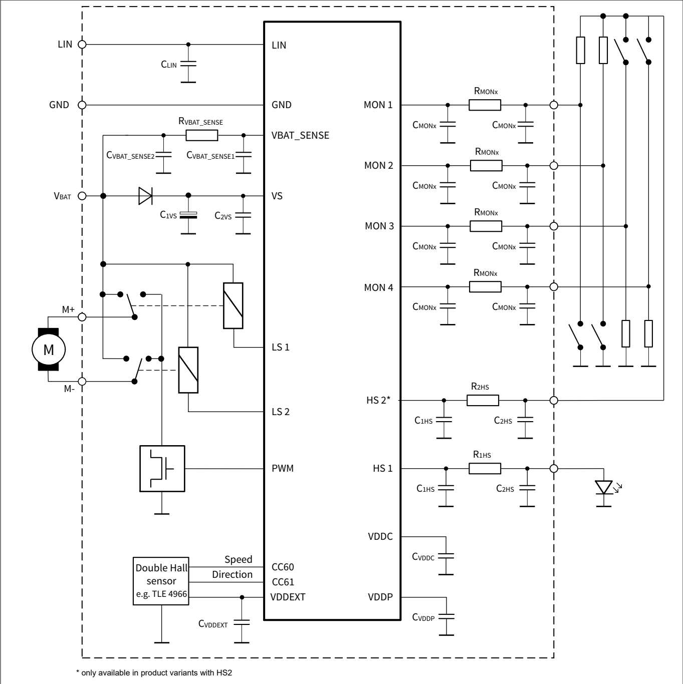
Figure 1 Typical application
