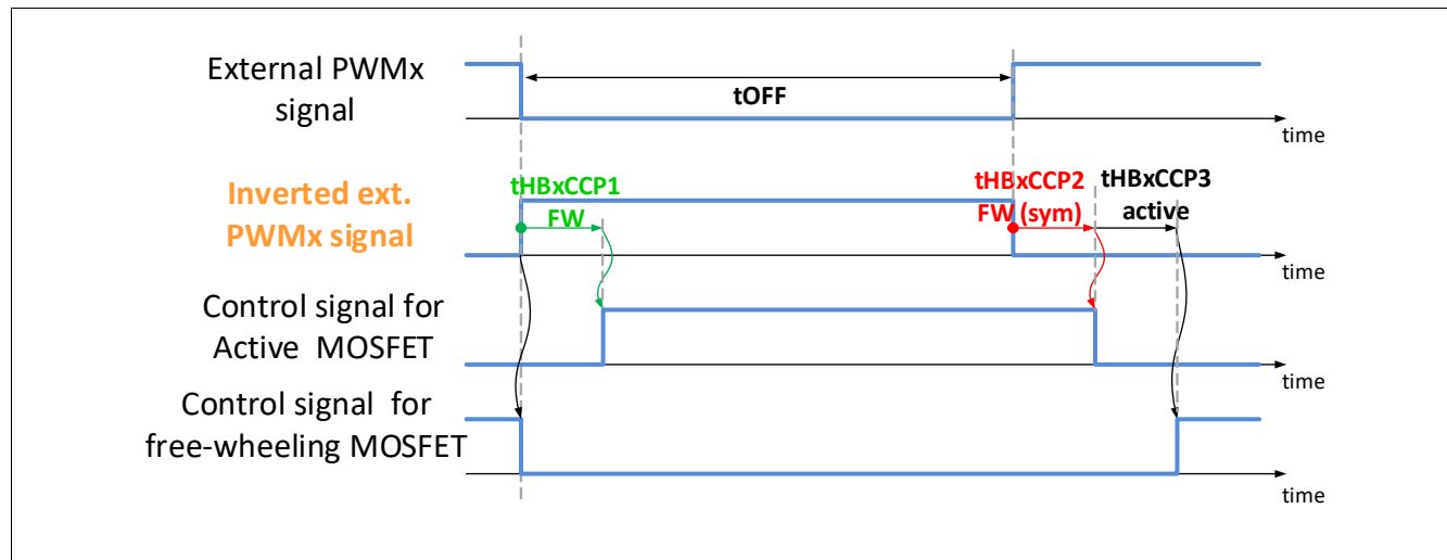
Figure 65 Internal signals for PWM operation - General case: t_{OFF} > t_{HBxCCP1} , t_{ON} > t_{HBxCCP1} + t_{HBxCCP2} , Motor operating as generator
