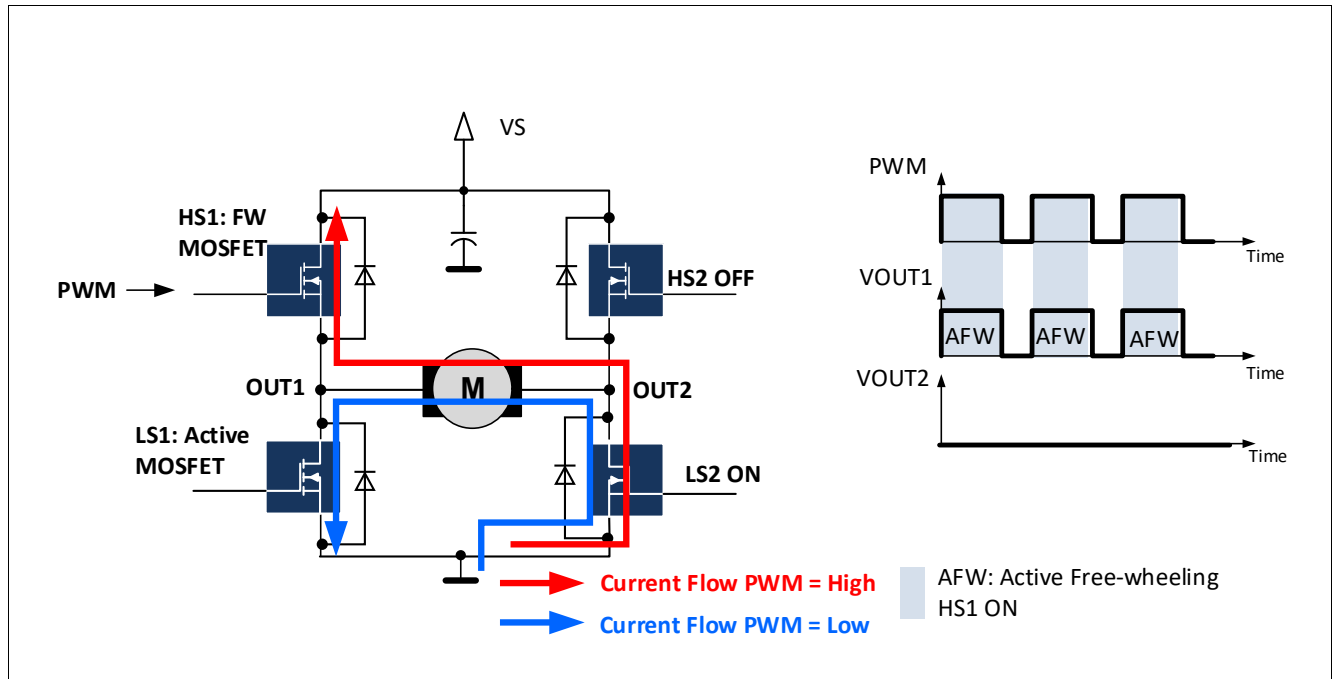
Figure 43 Active freewheeling on HB1: AFW1 = 1, HB1_PWM_EN = 1. PWM applied to HS1 (HB1MODE[1:0] = 10 B ), EN_GEN_CHECK = 1. The motor operates as generator: LS1 is the active MOSFET, HS1 is the FW MOSFET.
