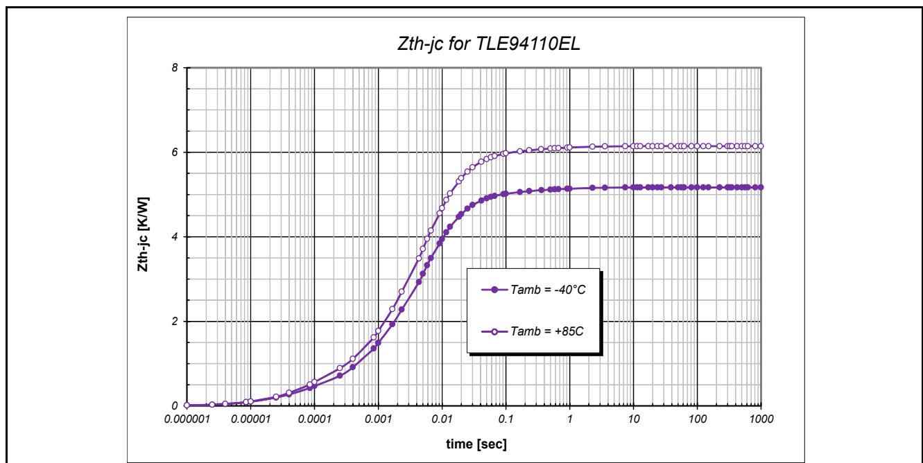
Figure 30 ZthJC Curve
