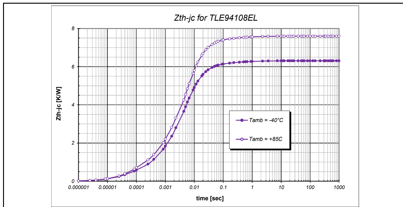
Figure 30 ZthJC Curve
