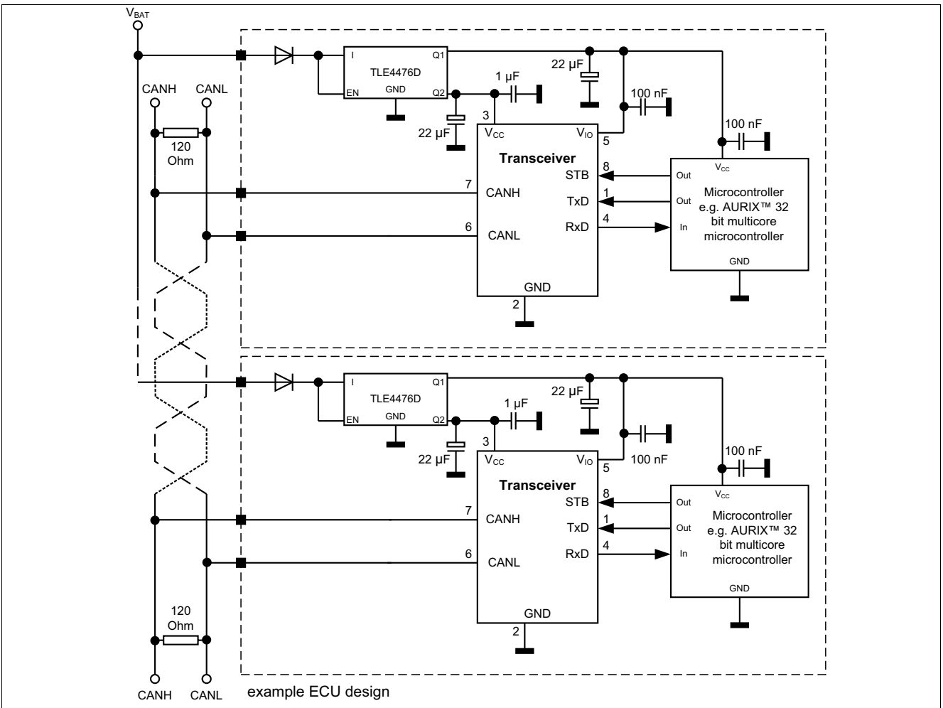
Figure 14 Application circuit
