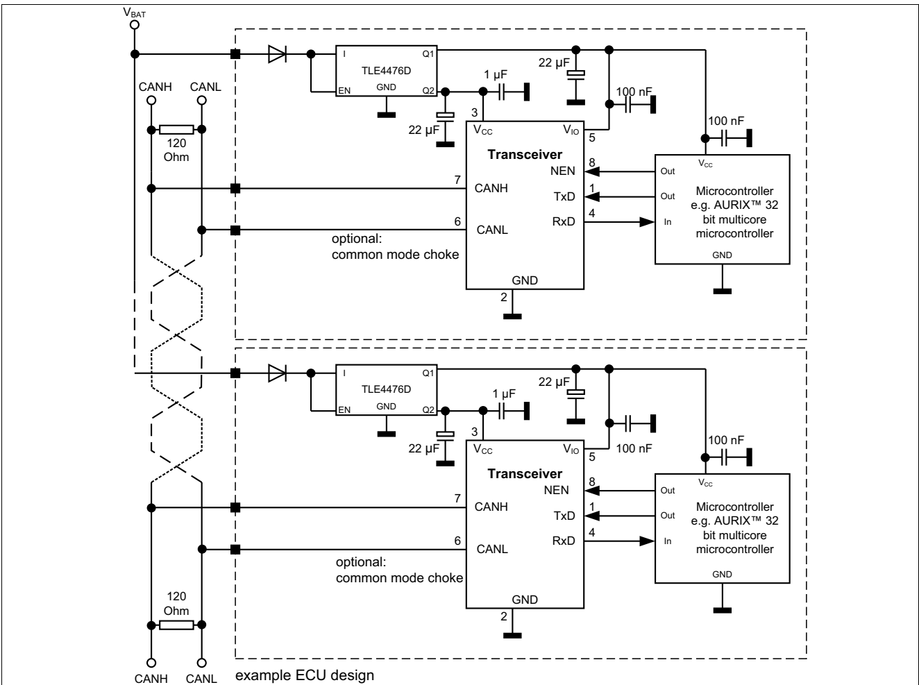
Figure 13 Application circuit
