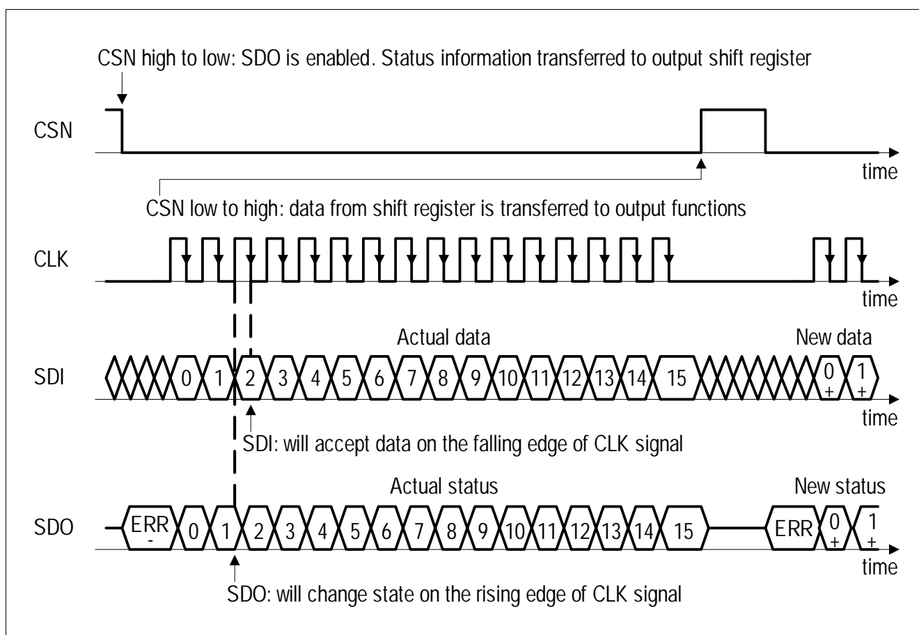
Figure 48 SPI Data Transfer Timing (note the reversed order of LSB and MSB shown in this figure compared to the register description)
