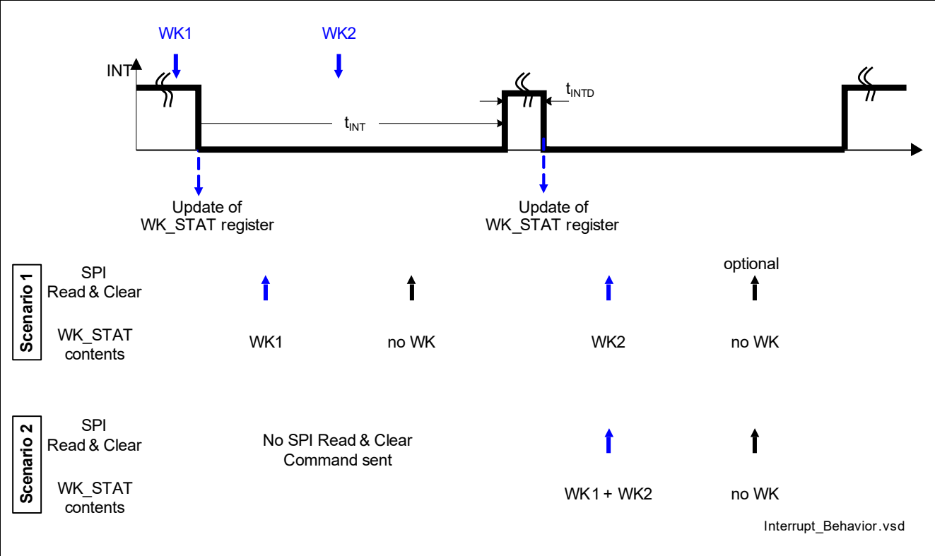
Figure 37 Interrupt Signaling Behavior
