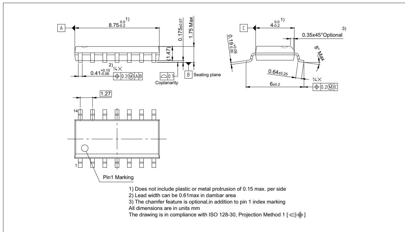
Figure 54 PG-DSO-14
