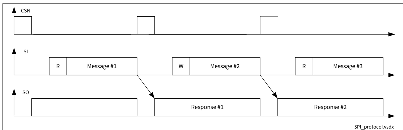
Figure 25 SPI protocol
