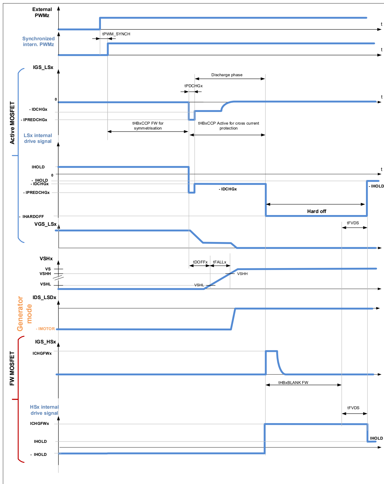
Figure 21 Adaptive turn-on, high-side PWM, AGC[1:0] = (1,0) or (1,1), motor operating as generator
