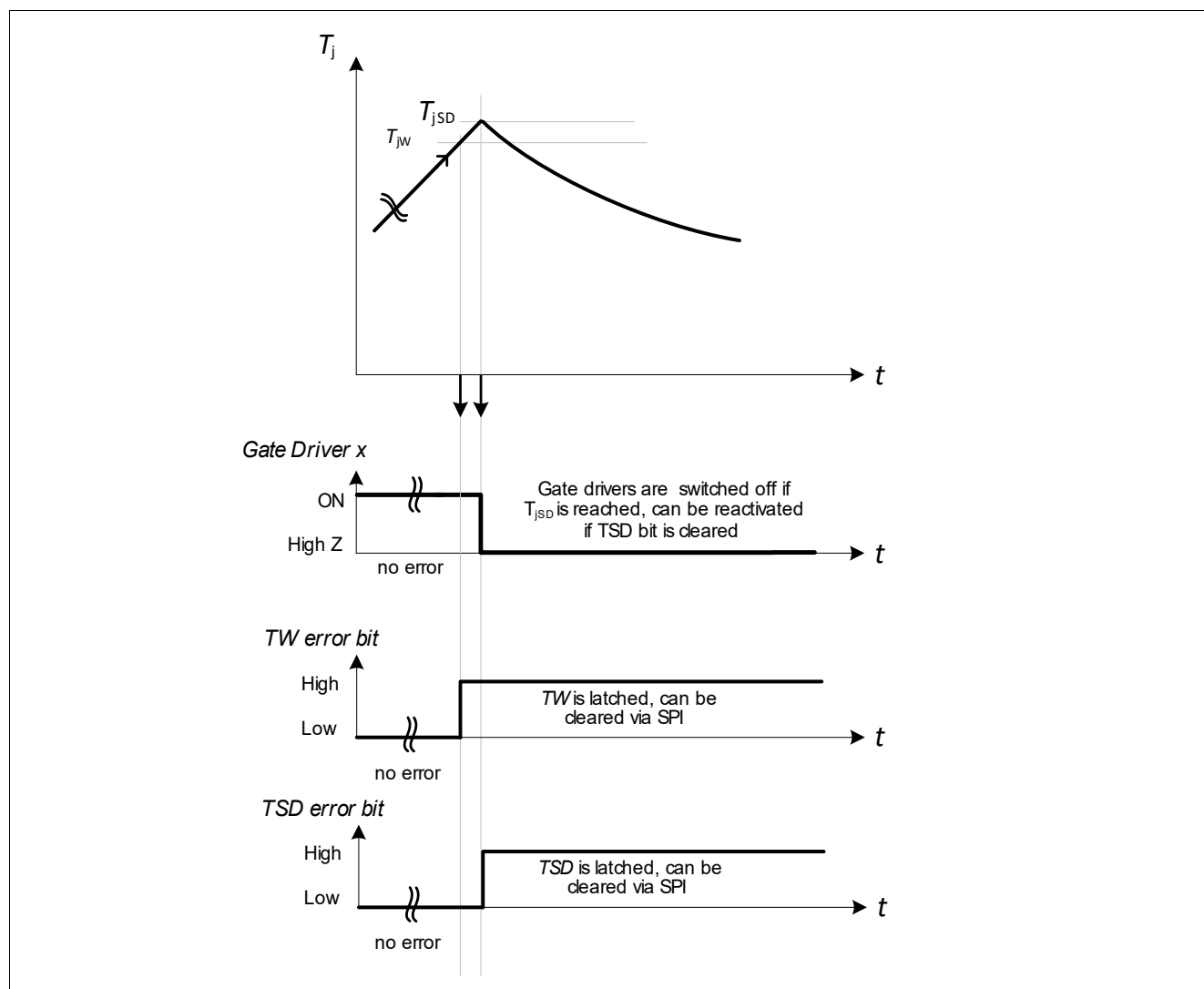
Figure 36 Overtemperature behavior
