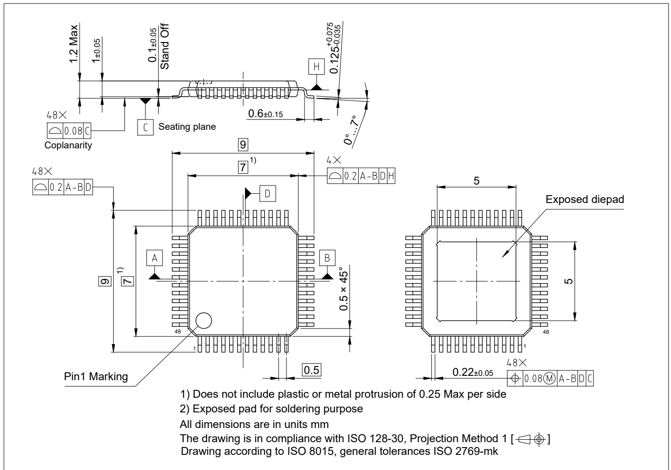
Figure 8 PG-TQFP-48
