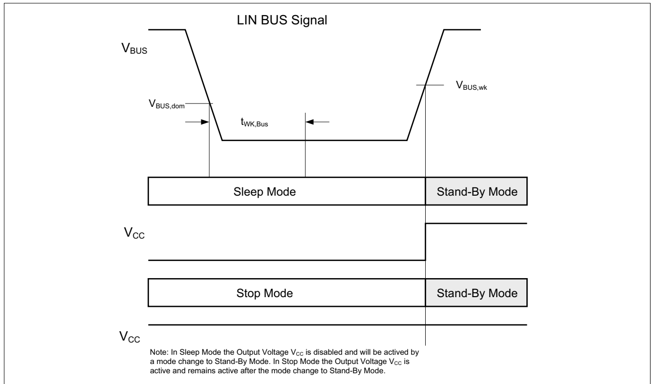
Figure 6 Bus Wake-up
