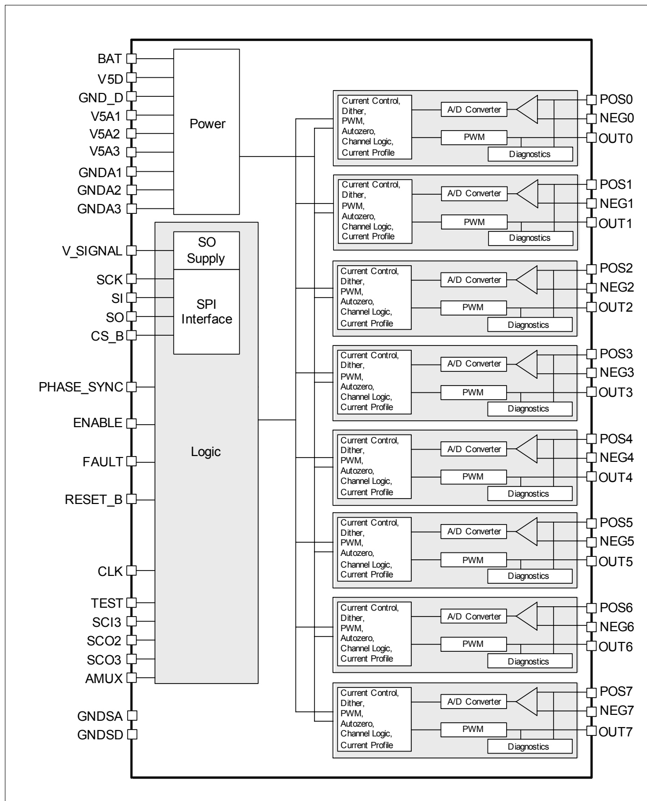
Figure 5 Block Diagram
