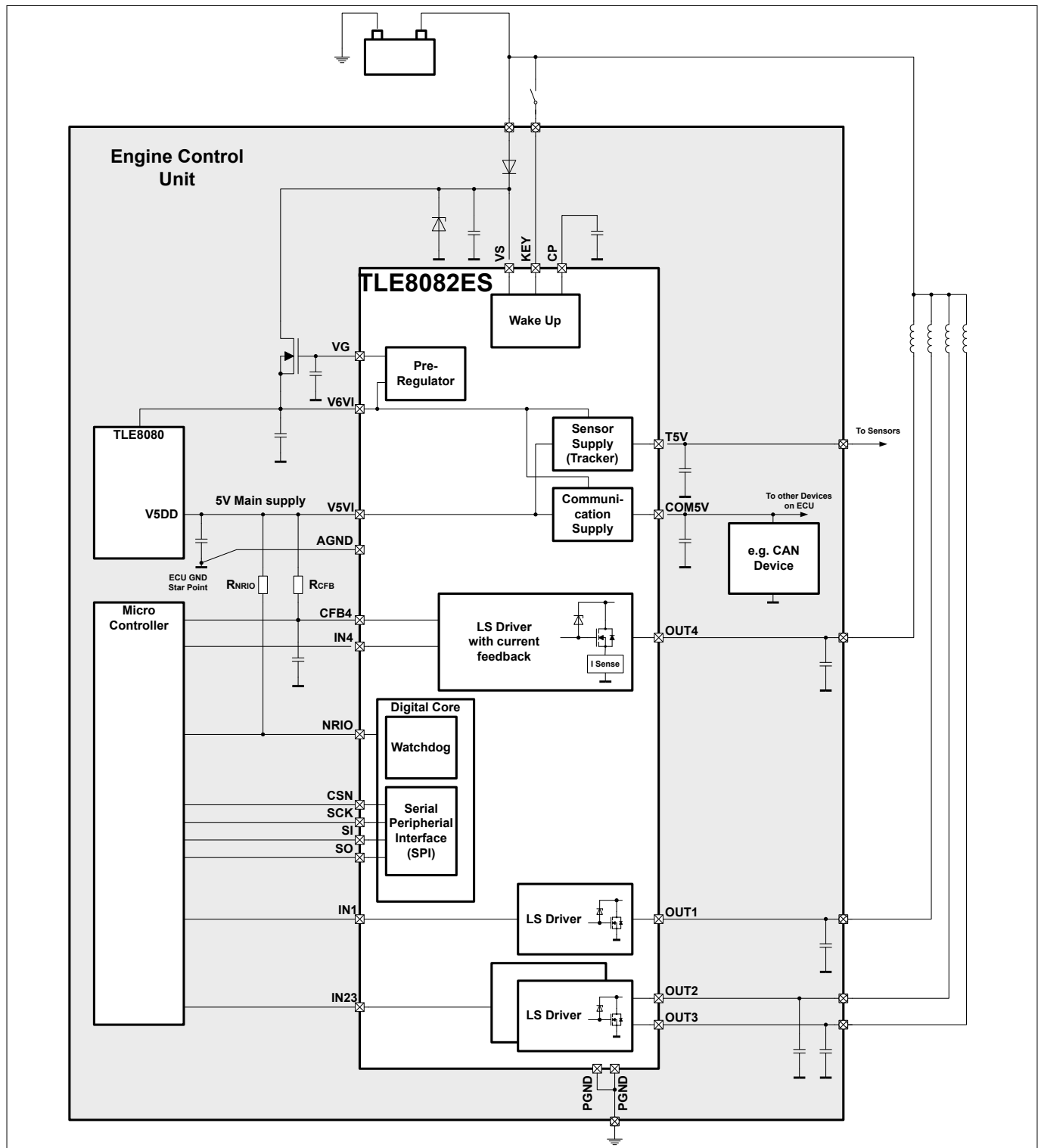
Figure 17 Application diagram
