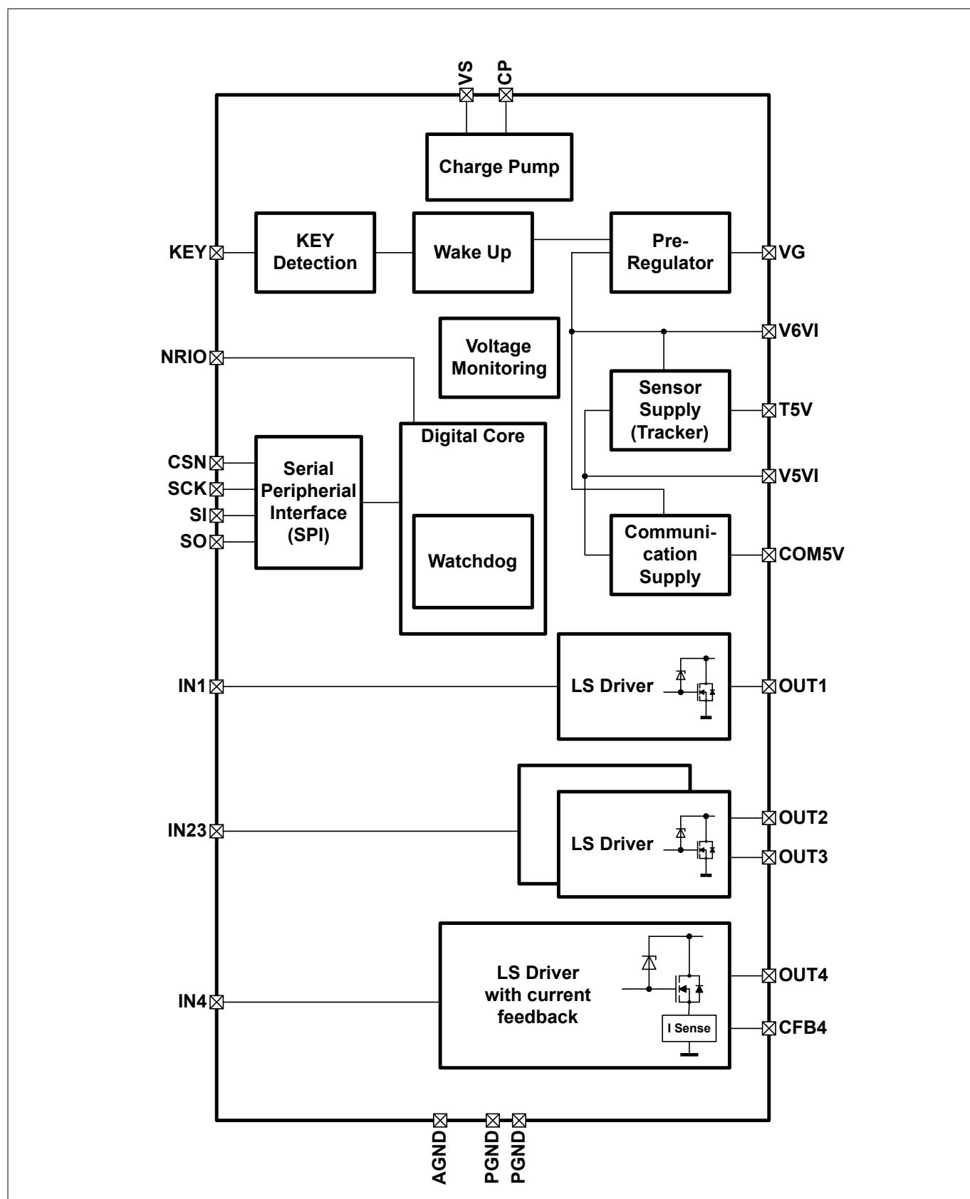
Figure 1 Block diagram
