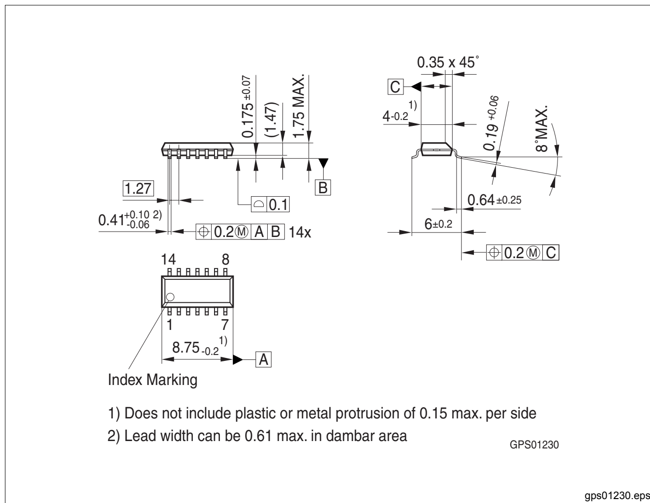
Figure 8 PG-DSO-14
