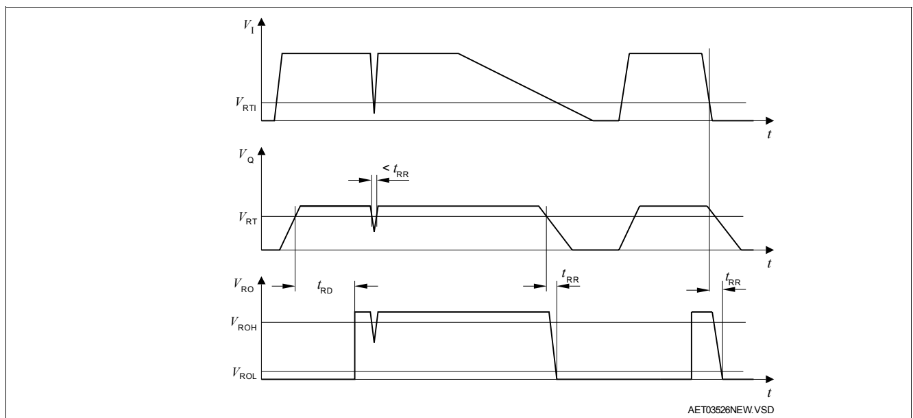
Figure 4 Reset Function and Timing Diagram
