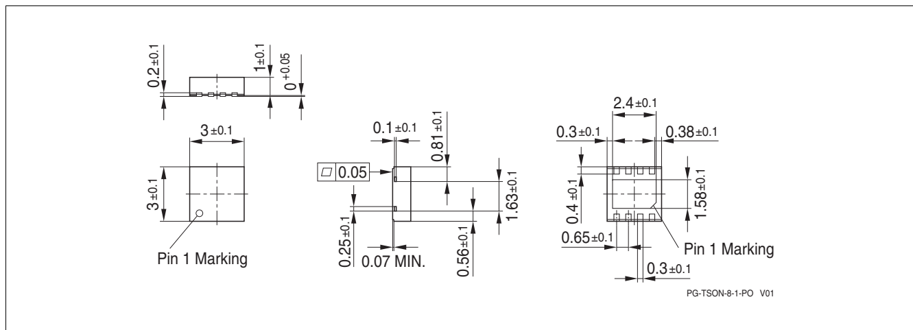
Figure 21 PG-TSON-8 (Plastic thin small outline nonleaded PG-TSON-8)
