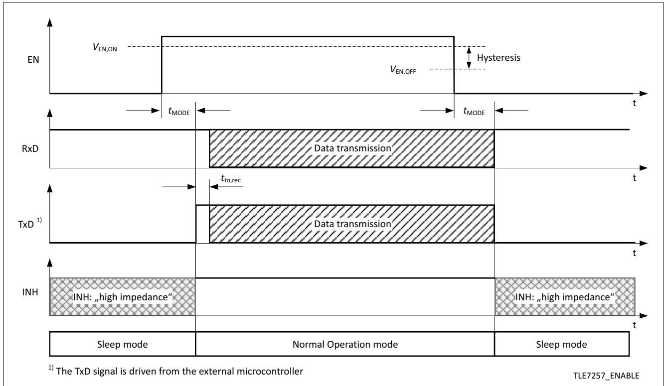
Figure 9 Entering Normal Operation mode from Sleep mode
