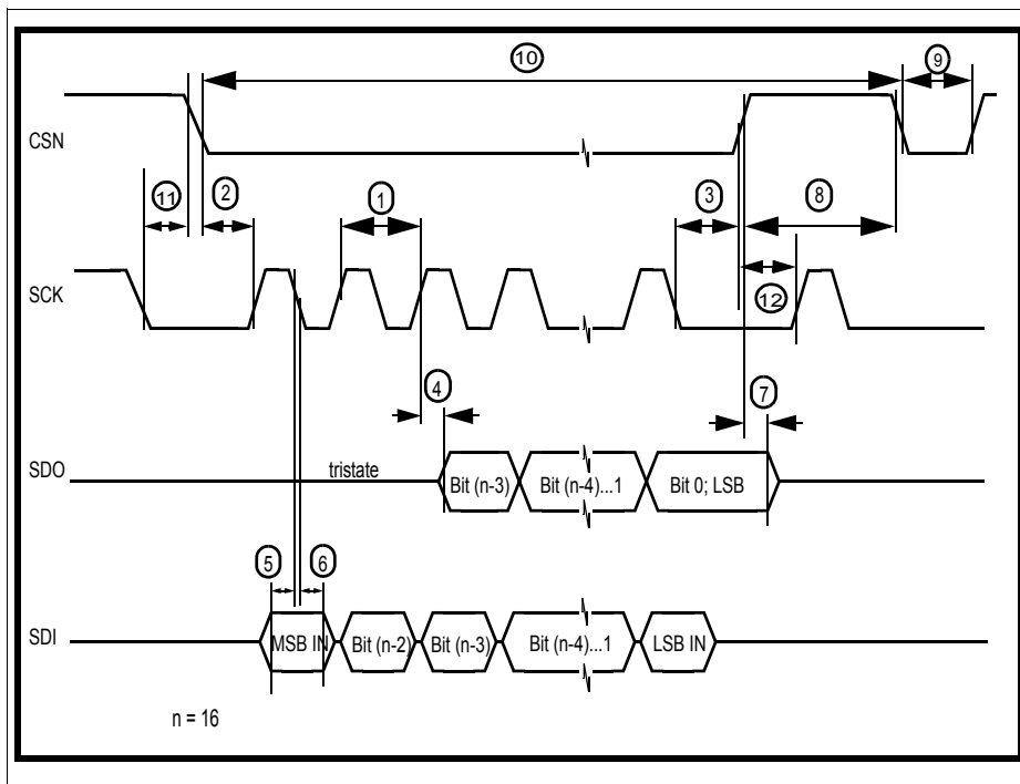
Figure 13 SPI-timing
