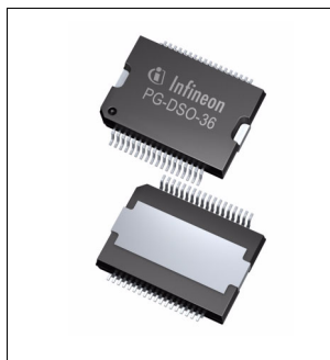
PG-DSO-36-26
