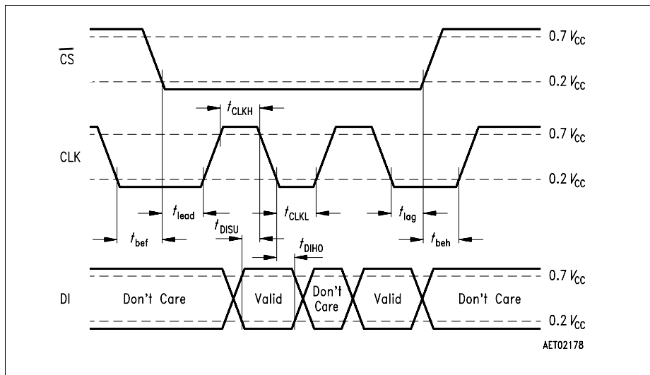
Figure 11 SPI-Input Timing
