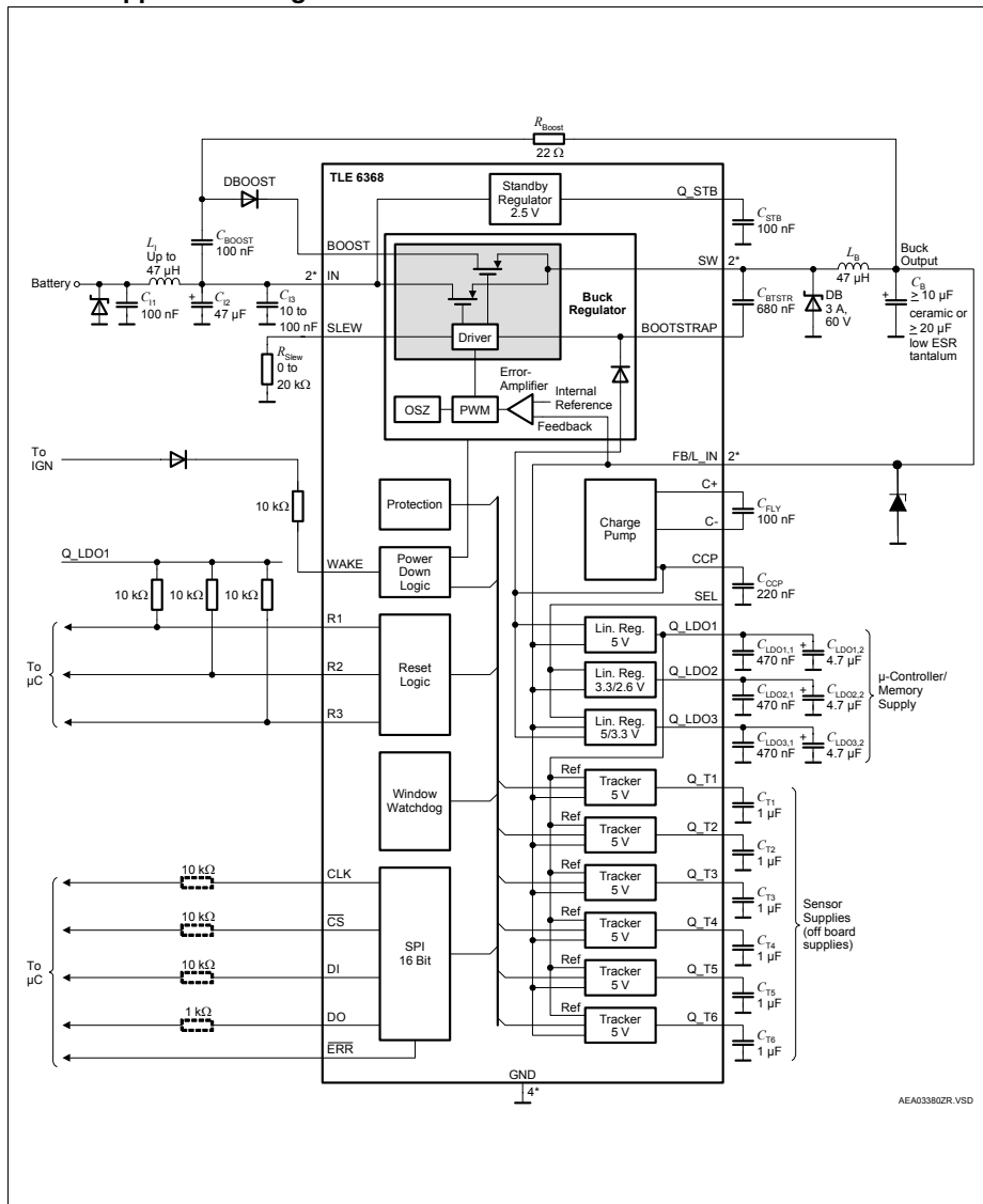
Figure 14 Application Diagram
