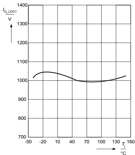
Q_LDO1 current limit vs. junction temperature
