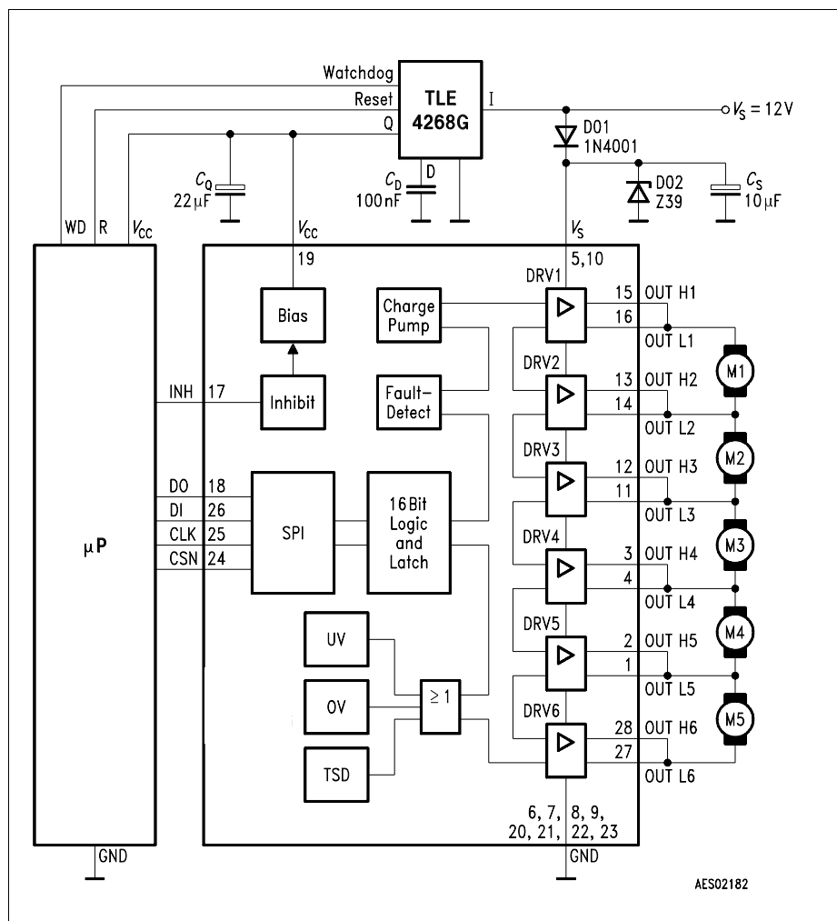
Figure 10 Application Circuit
