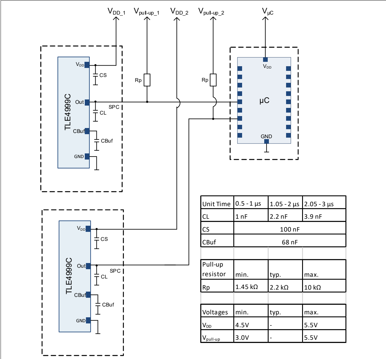
Figure 4 Application circuit
