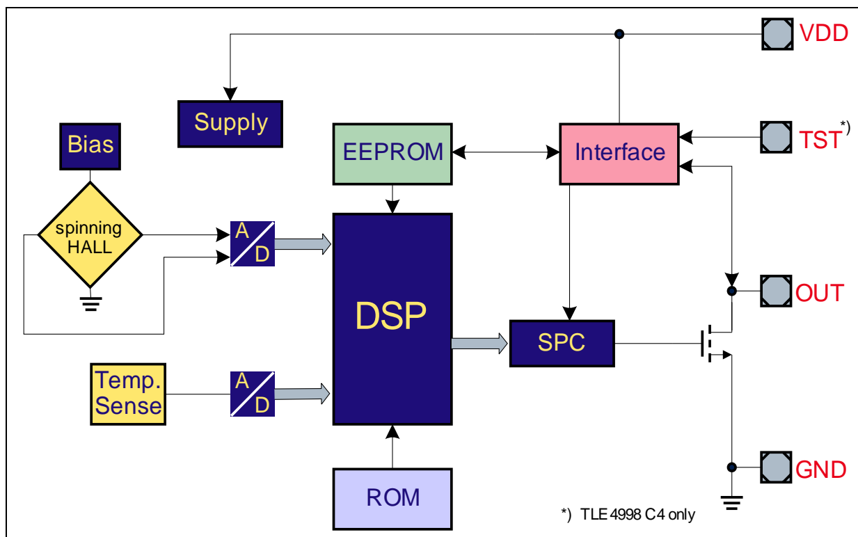
Figure 2 Block diagramm
