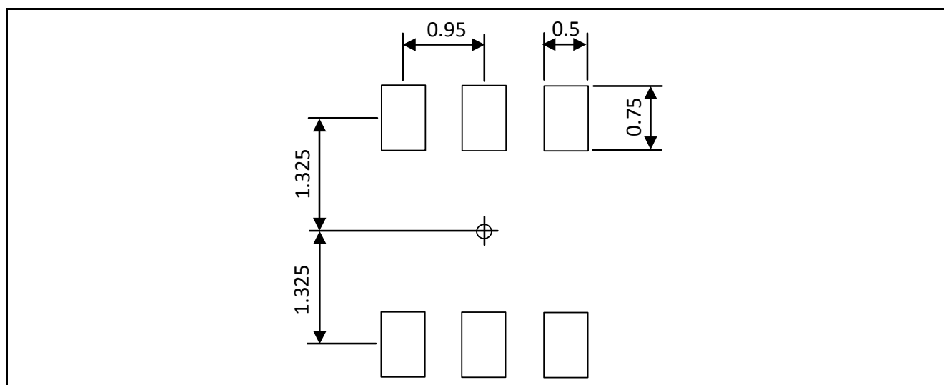
Figure 5-4 Footprint of PG-TSOP6-6-9
