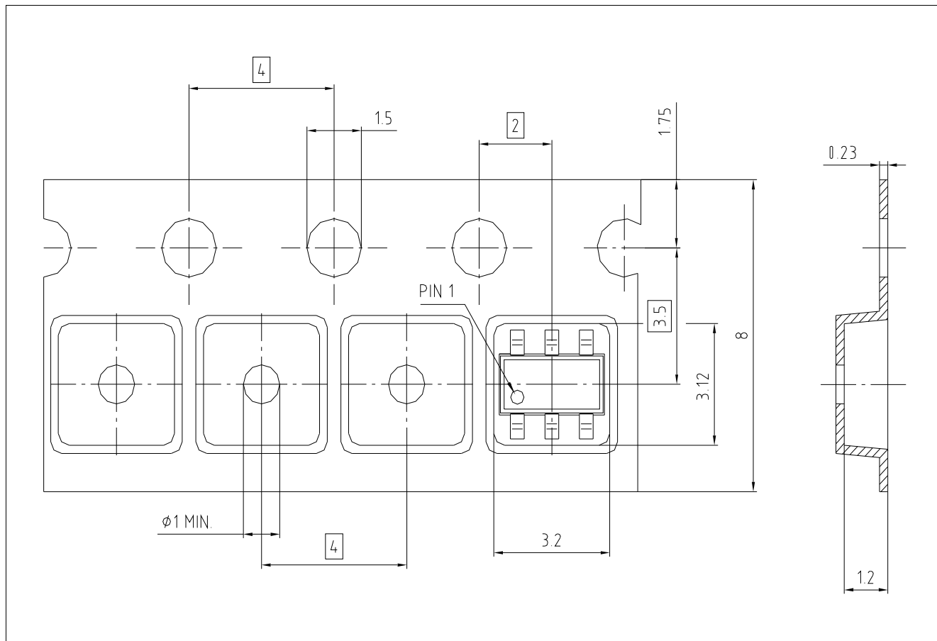
Figure 5-3 PG-TSOP6-6-9 Packing (All dimensions in mm)
