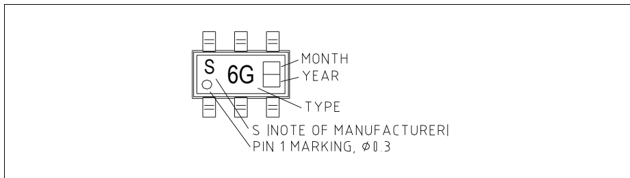
Figure 6 Marking PG-TSOP6-6-9
