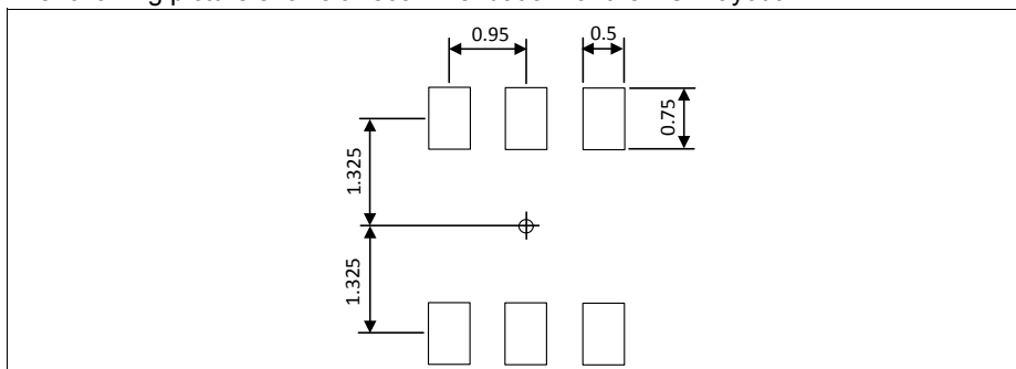
Figure 9 Footprint PG-TSOP6-9
