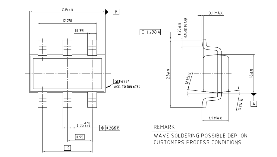
Figure 8 PG-TSOP6-9 (Plastic Thin Small Outline Package)
