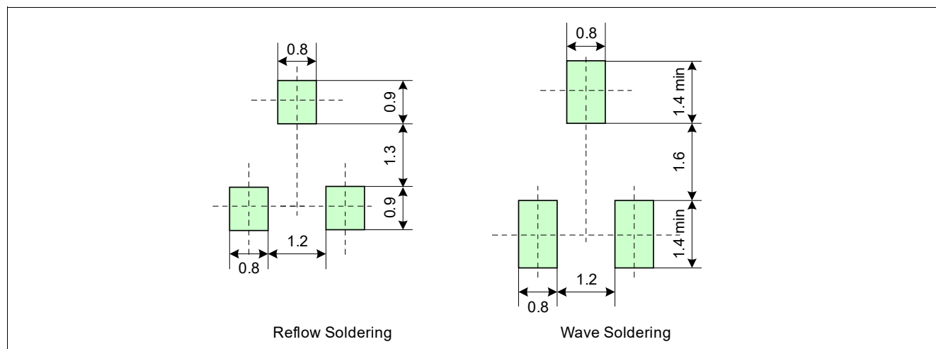
Figure 11 Footprint PG-SOT23-3-15
