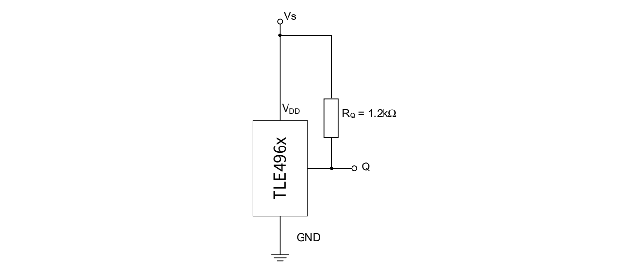
Figure 7 Application circuit
