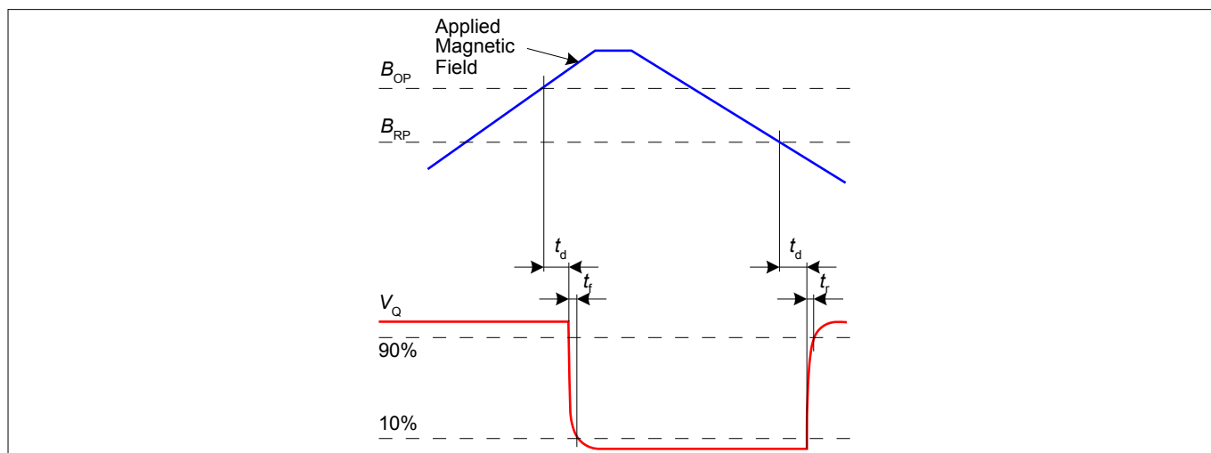
Figure 3 Timing diagram
