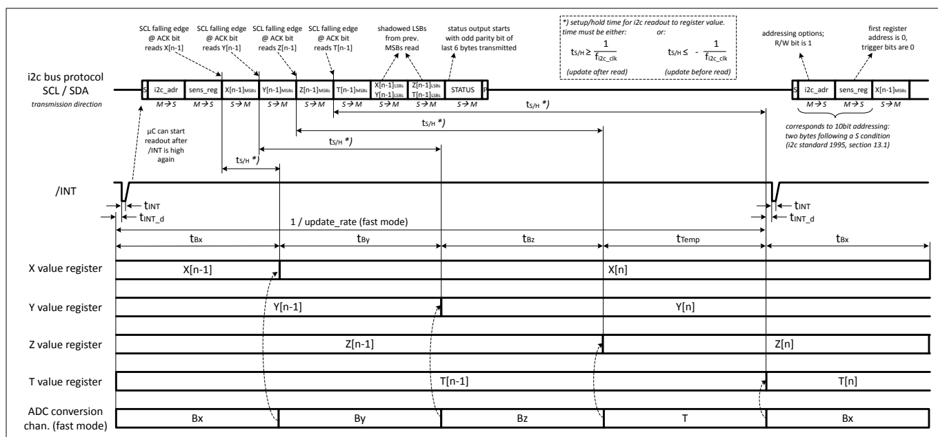
Figure 7 I 2 C readout frame, ADC conversion and related timing
