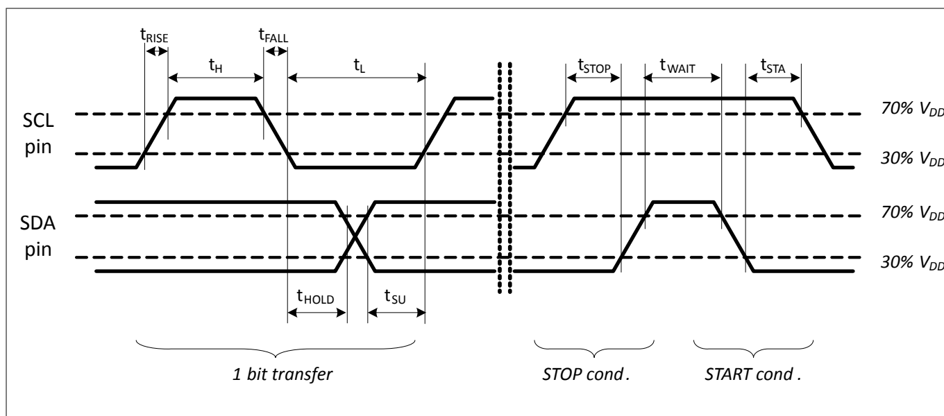
Figure 8 I 2 C timing specification
