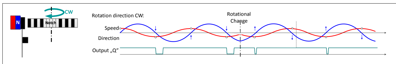
Figure 16 Signal output in setting “EDGE_POLAR = 1” and “FORWARD_DEF” = 1
