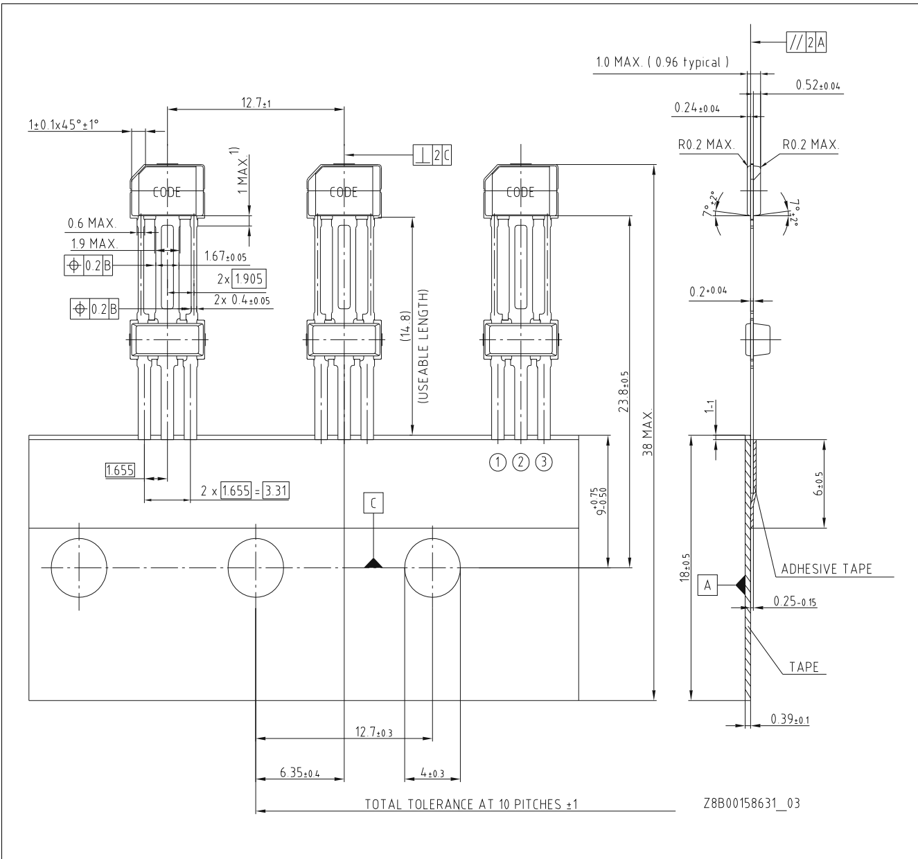
Figure 22 PG-SSO-3-5x Ammopack
