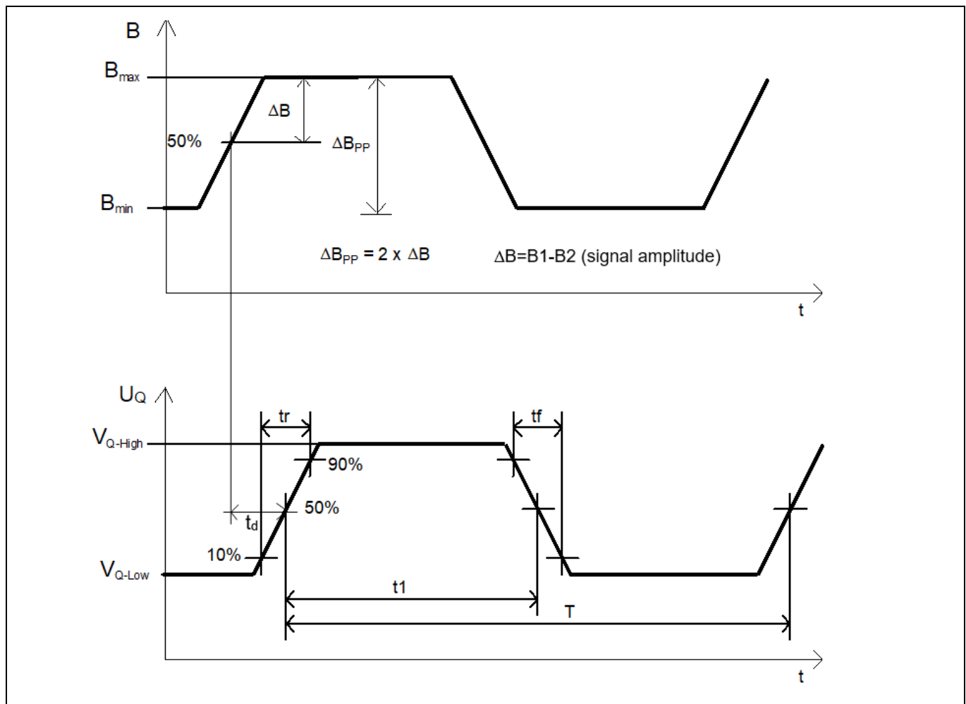
Figure 4 Switching direction
