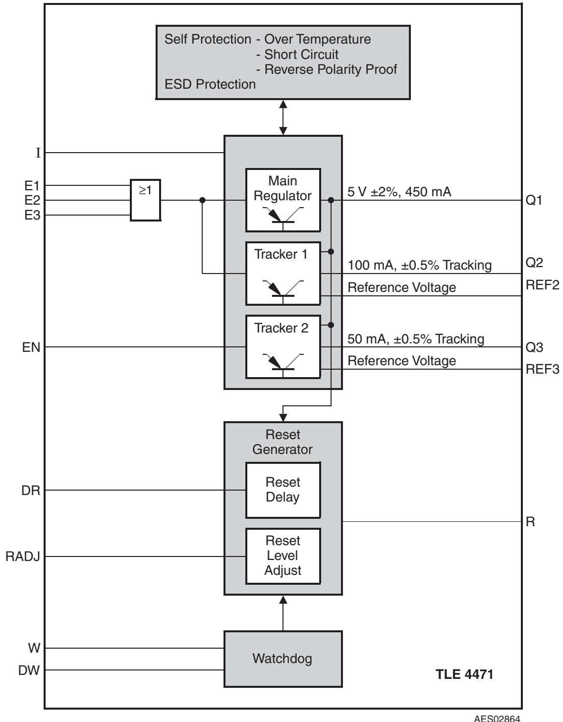
Figure 1 Block Diagram
