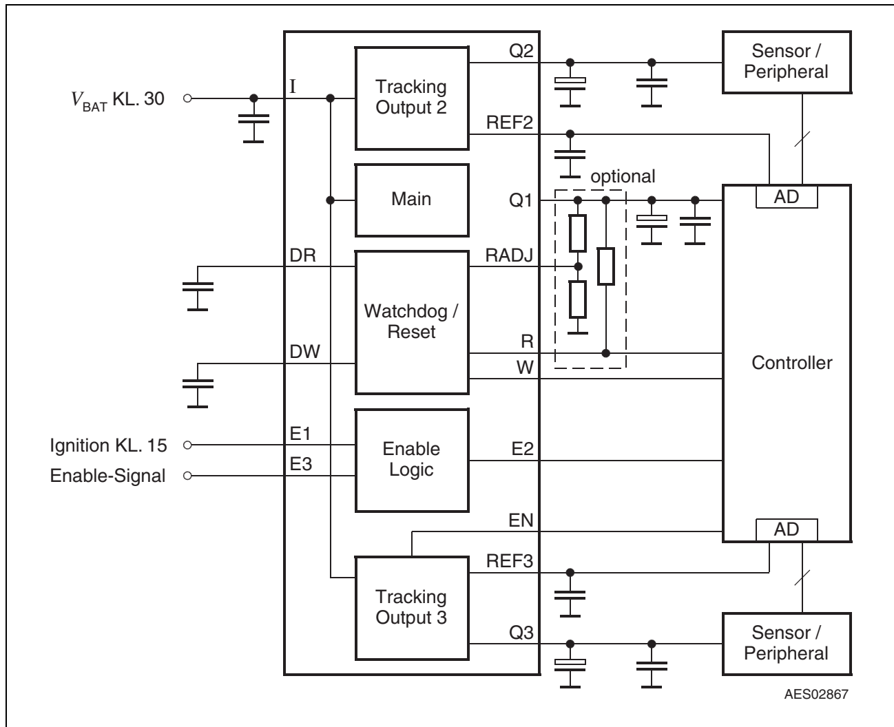
Figure 4 Application Diagram
